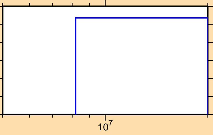
\sigma vs. E for ^{165}\text{Re}(n,2n)
