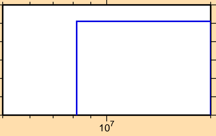
\sigma vs. E for ^{165}\text{Re}(n,2np)
