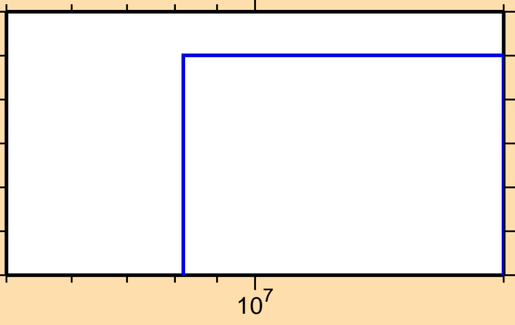
\sigma vs. E for ^{165}\text{Re}(n,2n\alpha)
