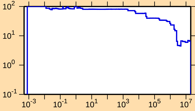
\Delta\sigma/\sigma vs. E for ^{165}\text{Re}(n,\text{nonel.})
