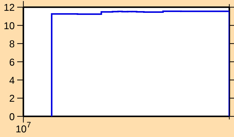
\Delta\sigma/\sigma vs. E for ^{165}\text{Re}(n,\text{el.})
