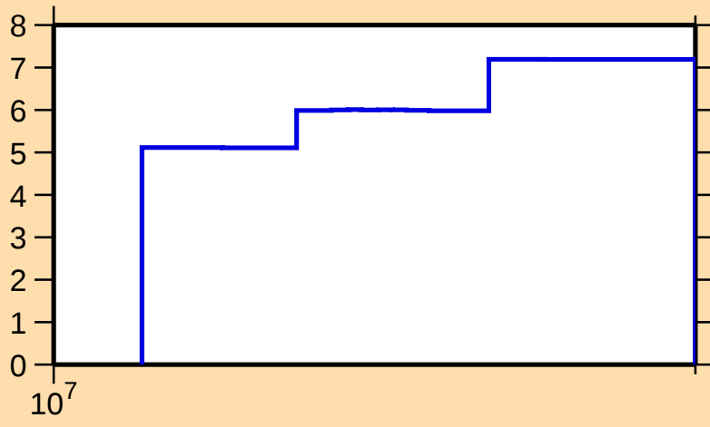
\Delta\sigma/\sigma vs. E for ^{165}\text{Re}(n,\text{tot.})
