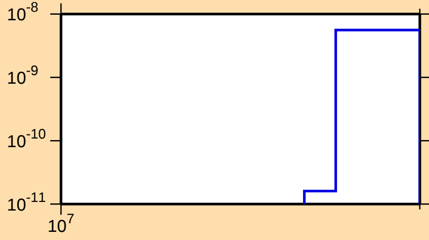
\sigma vs. E for ^{165}\text{Re}(n,nt)
