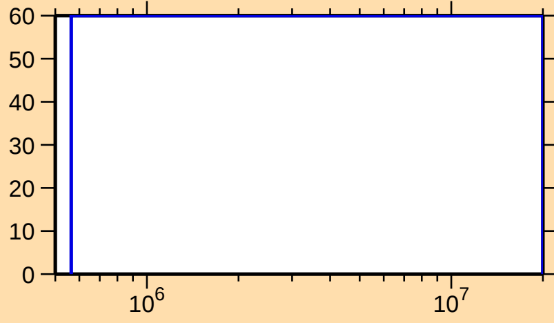
\Delta\sigma/\sigma vs. E for ^{165}\text{Re}(n,n\text{cont.})
