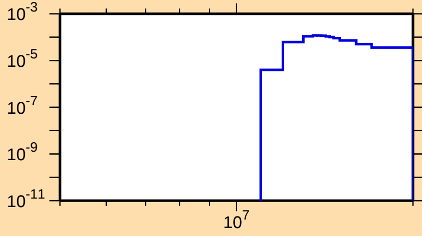
\sigma vs. E for ^{165}\text{Re}(n,2n\alpha)
