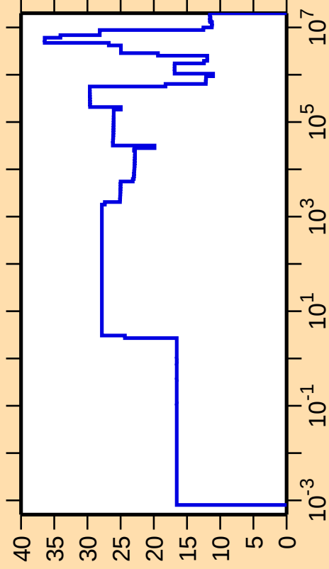
\Delta\sigma/\sigma vs. E for ^{165}\text{Re}(n,\text{el.})
