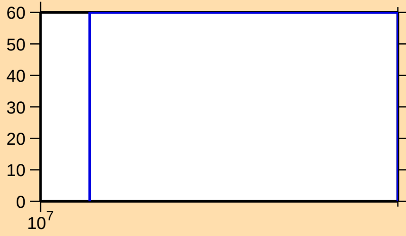
\Delta\sigma/\sigma vs. E for ^{165}\text{Re}(n,2n)
