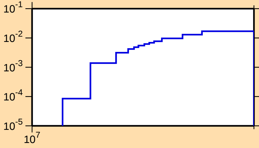
\sigma vs. E for ^{165}\text{Re}(n,2n)
