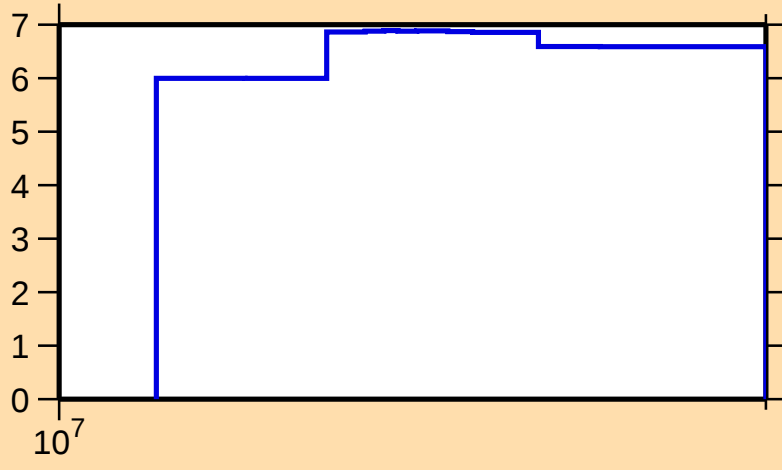
\Delta\sigma/\sigma vs. E for ^{165}\text{Re}(n,\text{nonel.})
