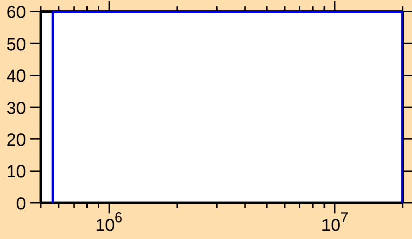
\Delta\sigma/\sigma vs. E for ^{165}\text{Re}(n,n\text{cont.})
