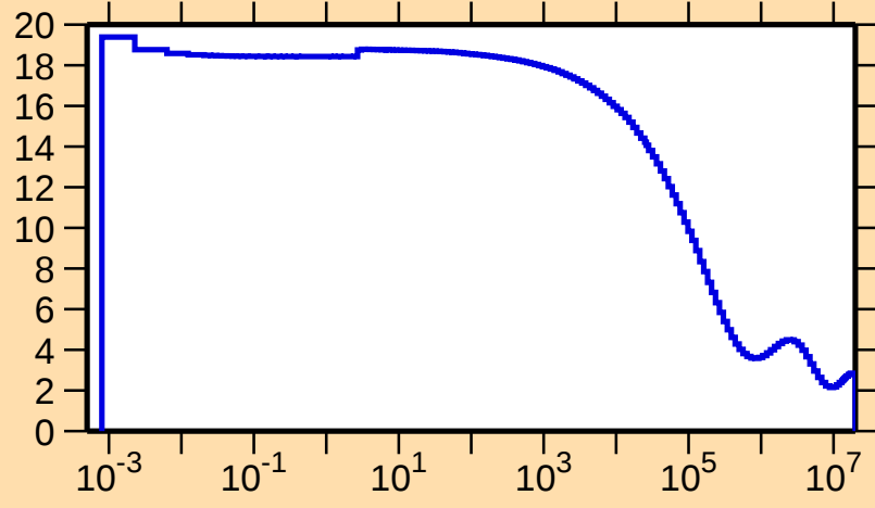
\sigma vs. E for ^{165}\text{Re}(n,\text{el.})
