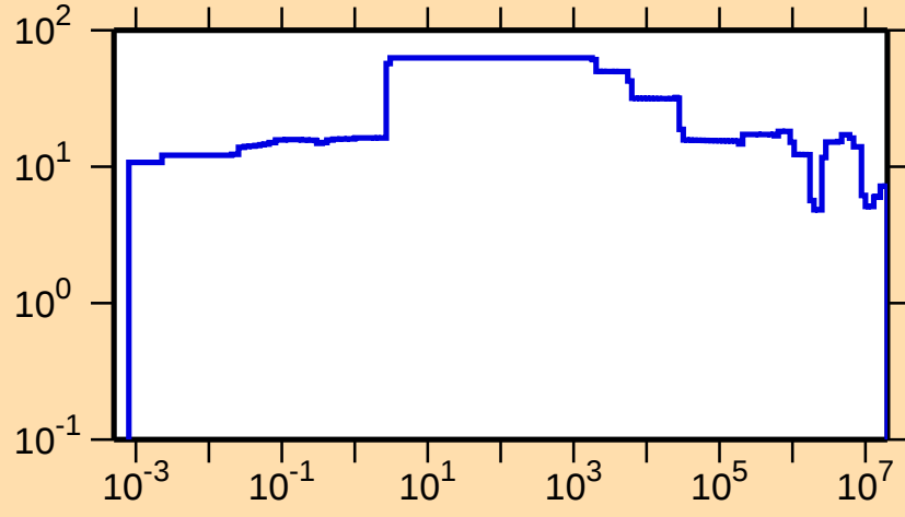
\Delta\sigma/\sigma vs. E for ^{165}\text{Re}(n,\text{tot.})
