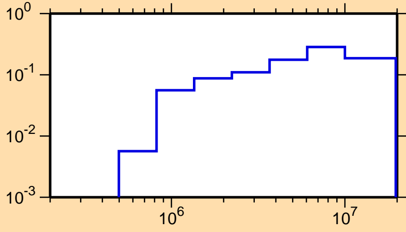
\sigma vs. E for ^{165}\text{Re}(n,n\text{cont.})
