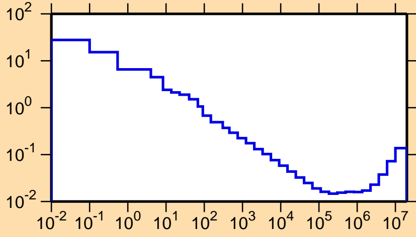
\sigma vs. E for ^{165}\text{Re}(n,\alpha)
