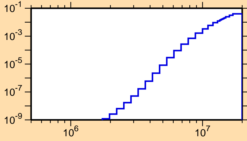
\sigma vs. E for ^{166}\text{Re}(n,n\alpha)
