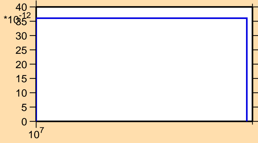
\sigma vs. E for ^{166}\text{Re}(n,nt)
