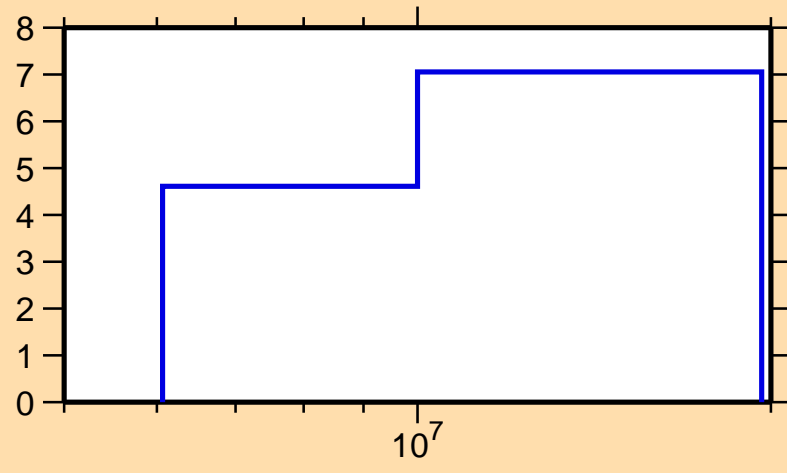
\Delta\sigma/\sigma vs. E for ^{166}\text{Re}(n,\text{nonel.})
