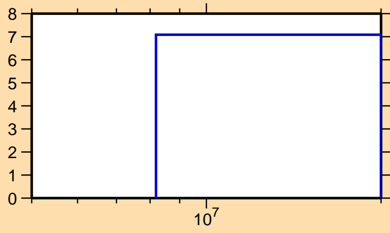
\Delta\sigma/\sigma vs. E for ^{166}\text{Re}(n,\text{tot.})
