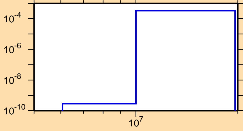
\sigma vs. E for ^{167}\text{Re}(n,t)
