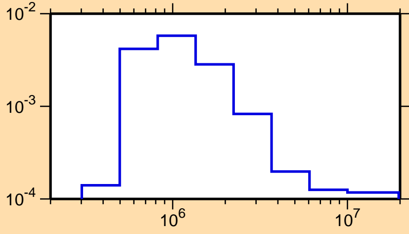
\sigma vs. E for ^{167}\text{Re}(n,n_4)
