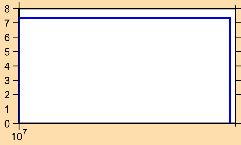
\Delta\sigma/\sigma vs. E for ^{167}\text{Re}(n,\text{el.})
