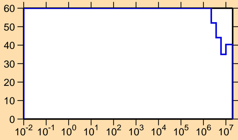
\Delta\sigma/\sigma vs. E for ^{167}\text{Re}(n,p)
