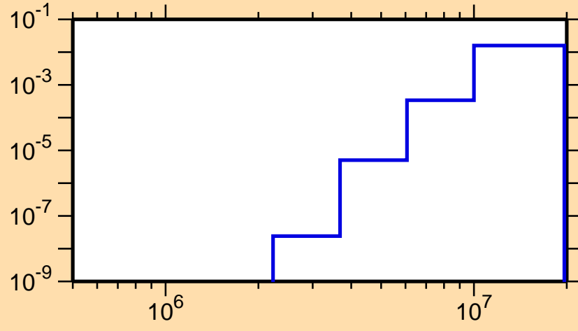
\sigma vs. E for ^{167}\text{Re}(n,n\alpha)
