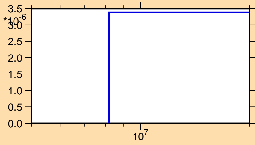
\sigma vs. E for ^{167}\text{Re}(n,\text{pd})
