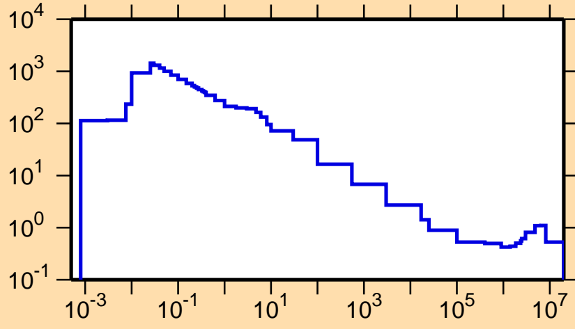
\sigma vs. E for ^{167}\text{Re}(n,p)
