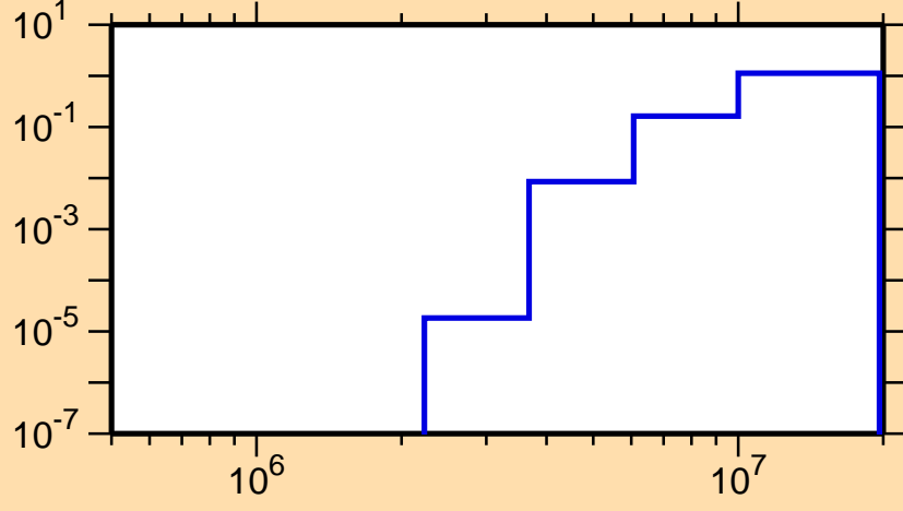
\sigma vs. E for ^{167}\text{Re}(n,np)
