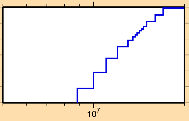
\sigma vs. E for ^{168}\text{Re}(\text{mt117})
