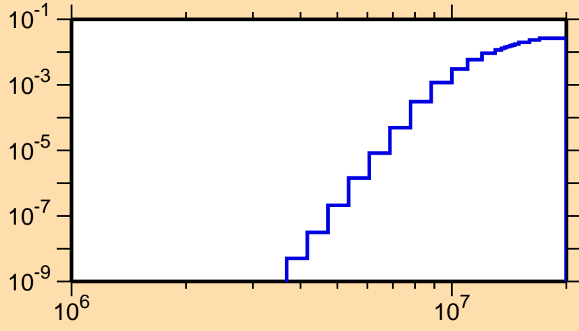
\sigma vs. E for ^{168}\text{Re}(n,d)
