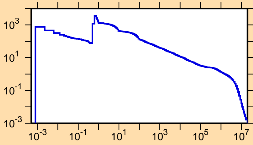
\sigma vs. E for ^{168}\text{Re}(n,\gamma)
