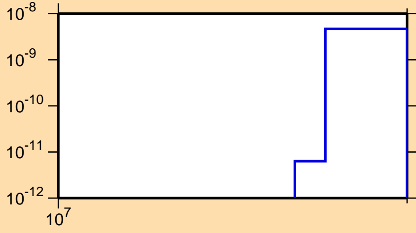
\sigma vs. E for ^{168}\text{Re}(n,nt)
