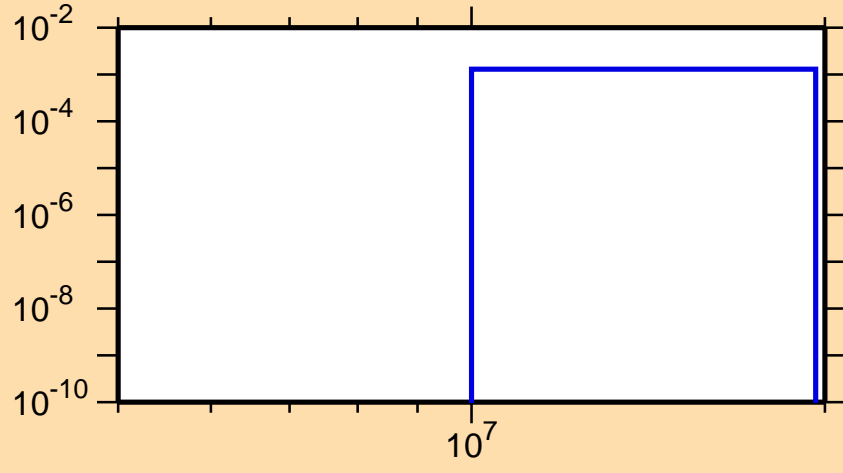
\sigma vs. E for ^{168}\text{Re}(n,2np)
