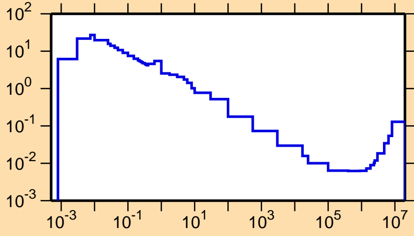
\sigma vs. E for ^{168}\text{Re}(n,\alpha)
