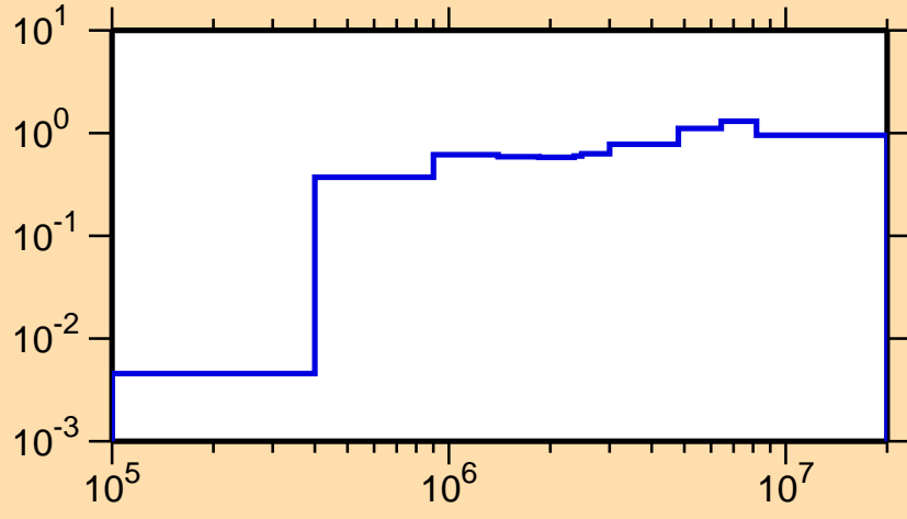
\sigma vs. E for ^{168}\text{Re}(n,\text{inel.})
