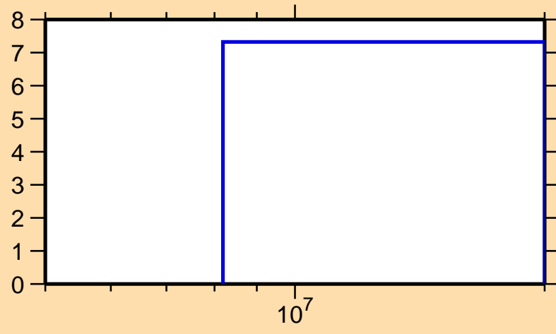
\Delta\sigma/\sigma vs. E for ^{168}\text{Re}(n,\text{tot.})
