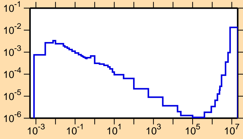
\sigma vs. E for ^{168}\text{Re}(n,p\alpha)
