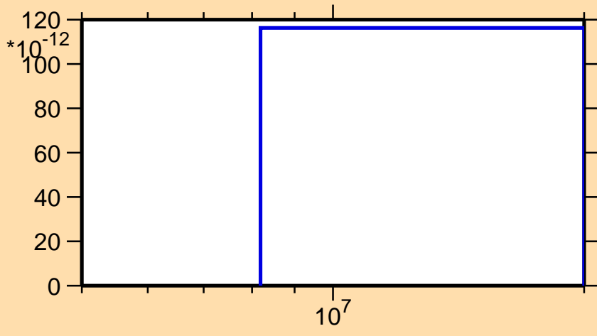
\sigma vs. E for ^{168}\text{Re}(\text{mt } 34)
