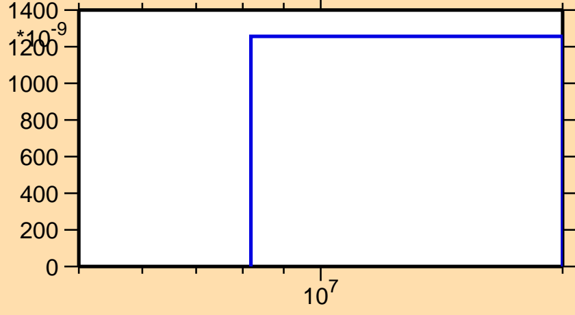
\sigma vs. E for ^{168}\text{Re}(n,\text{nd})
