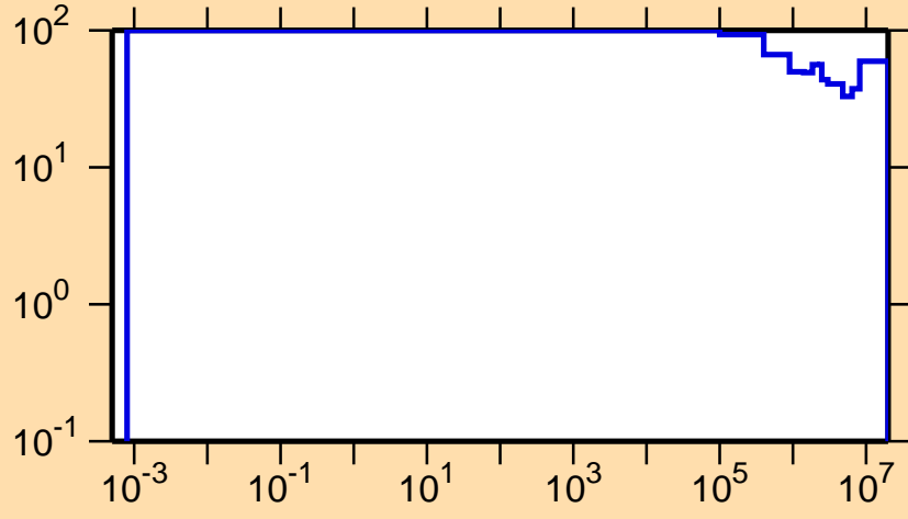
\Delta\sigma/\sigma vs. E for ^{168}\text{Re}(n,p)
