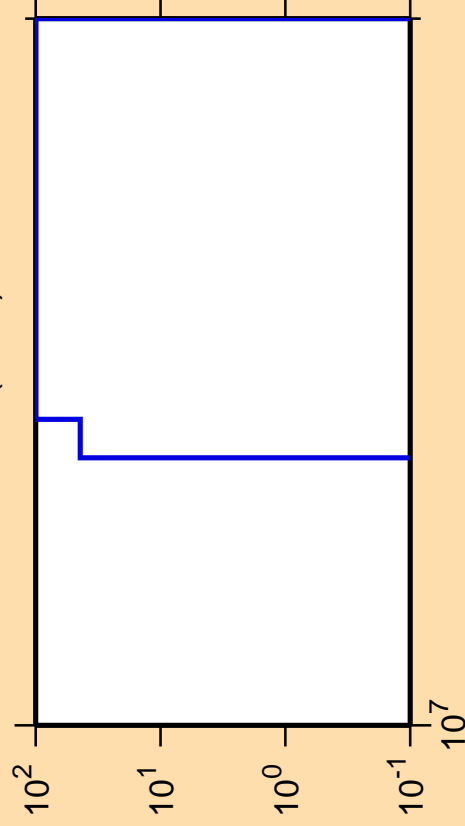
\Delta\sigma/\sigma vs. E for ^{169}\text{Re}(n,nd)
