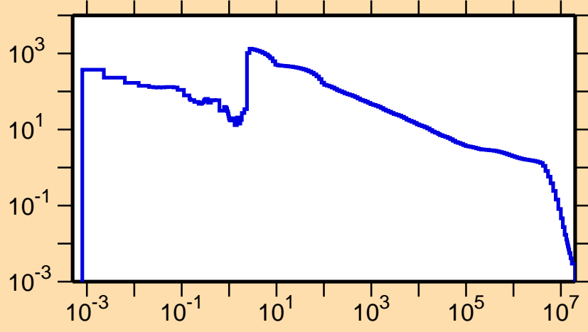
\sigma vs. E for ^{169}\text{Re}(n,\gamma)
