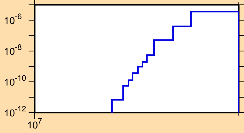
\sigma vs. E for ^{169}\text{Re}(n,nd)
