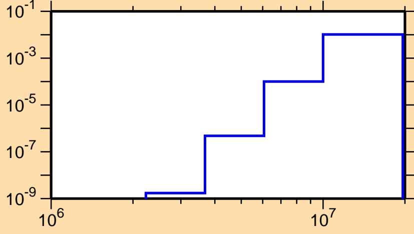
\sigma vs. E for ^{169}\text{Re}(n,d)
