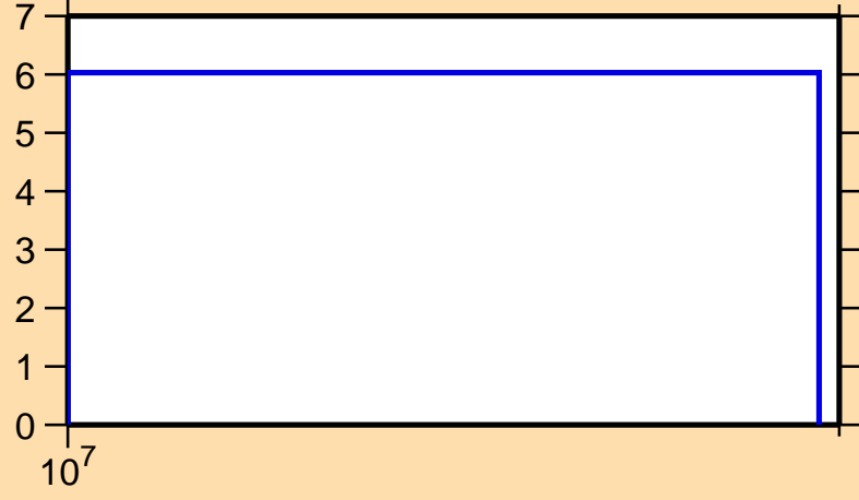
\Delta\sigma/\sigma vs. E for ^{169}\text{Re}(n,\text{tot.})
