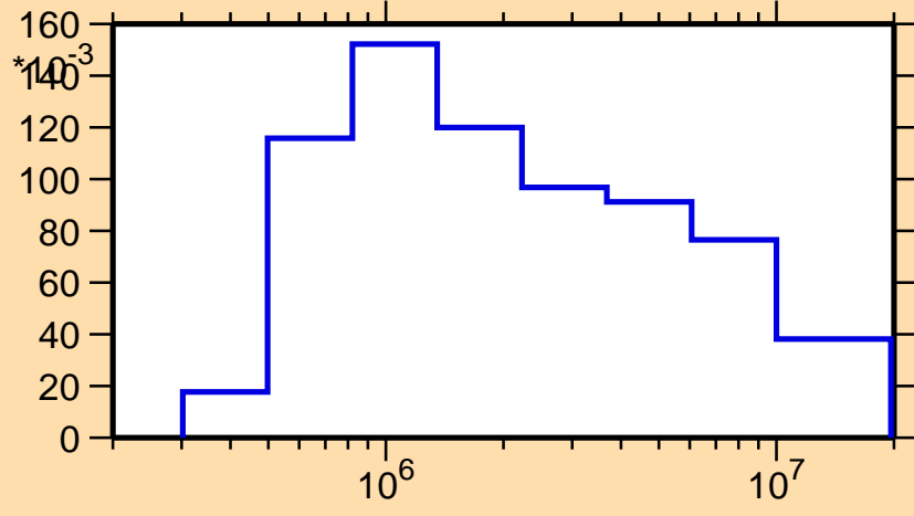
\sigma vs. E for ^{169}\text{Re}(n,n_3)
