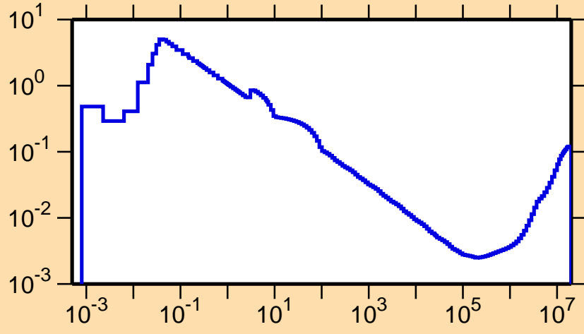
\sigma vs. E for ^{169}\text{Re}(n,\alpha)
