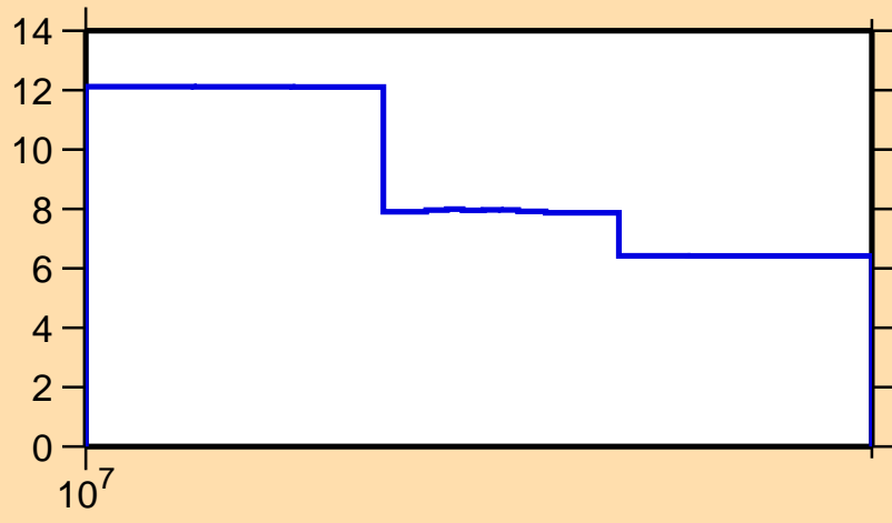
\Delta\sigma/\sigma vs. E for ^{169}\text{Re}(n,\text{el.})
