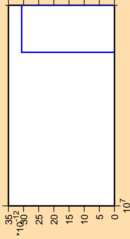
\Delta\sigma/\sigma vs. E for ^{169}\text{Re}(\text{mt } 42)
