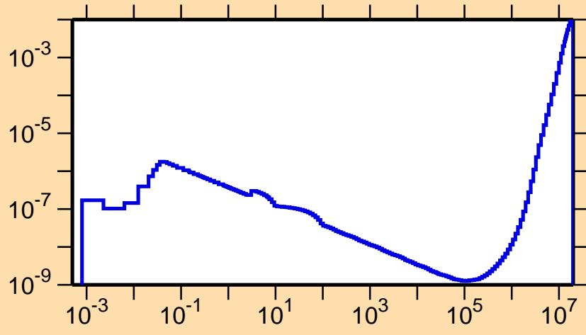
\sigma vs. E for ^{169}\text{Re}(n,p\alpha)
