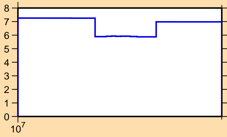
\Delta\sigma/\sigma vs. E for ^{169}\text{Re}(n,\text{tot.})
