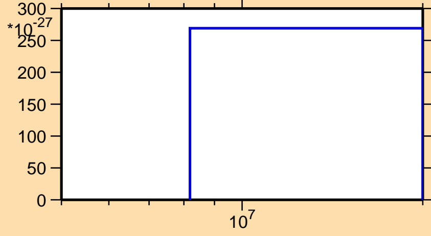
\sigma vs. E for ^{169}\text{Re}(\text{mt } 42)
