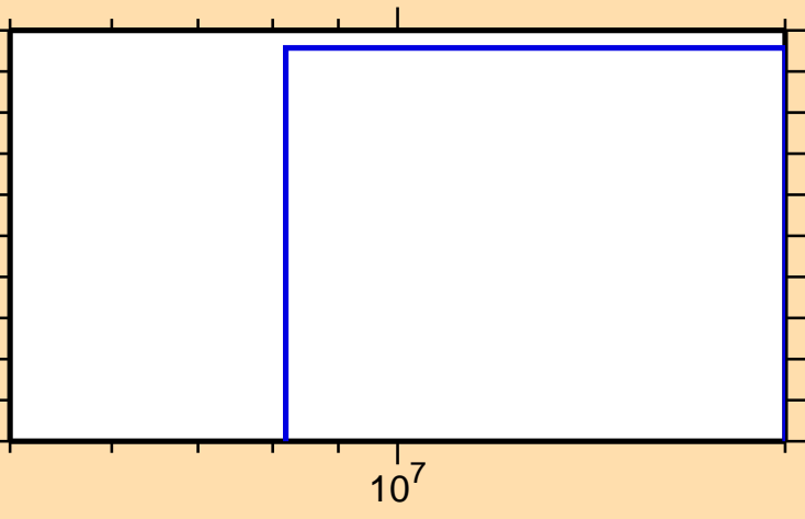
\sigma vs. E for ^{169}\text{Re}(n,\text{pt})
