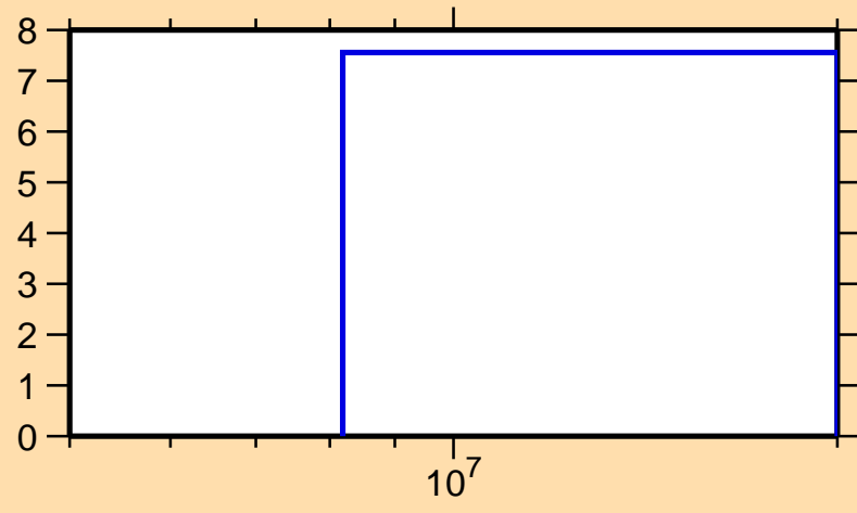
\Delta\sigma/\sigma vs. E for ^{169}\text{Re}(n,\text{el.})
