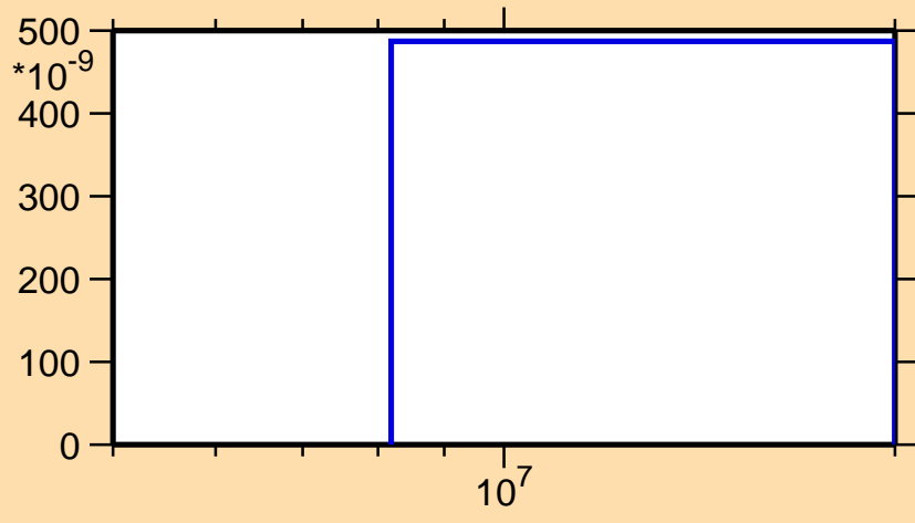
\sigma vs. E for ^{169}\text{Re}(n,\text{pd})
