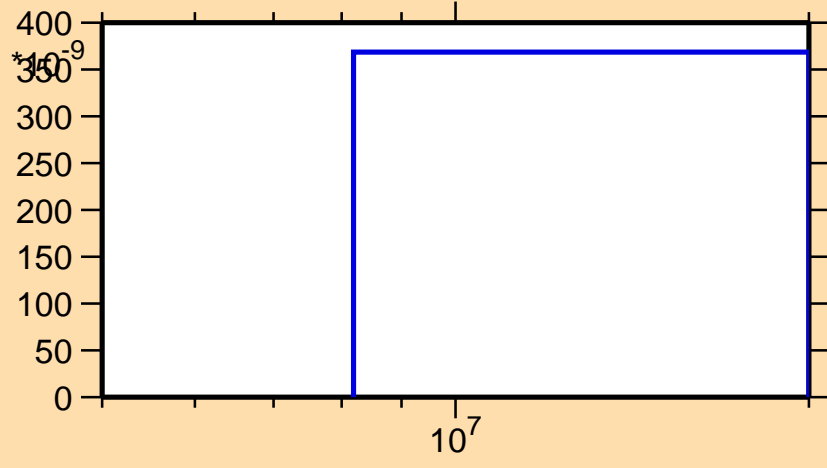
\sigma vs. E for ^{169}\text{Re}(n,2n\alpha)
