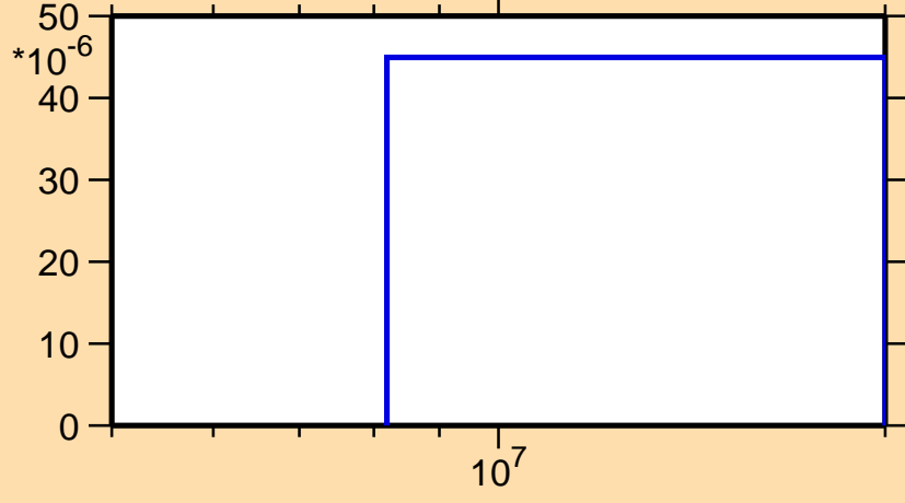
\sigma vs. E for ^{169}\text{Re}(n,2np)
