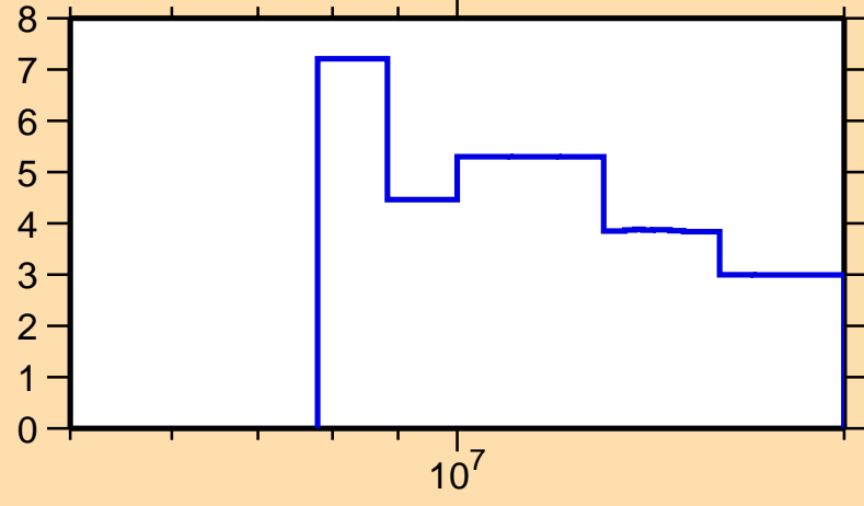
\Delta\sigma/\sigma vs. E for ^{170}\text{Re}(n,tot.)
