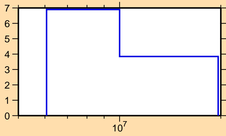
\Delta\sigma/\sigma vs. E for ^{170}\text{Re}(n,\text{tot.})
