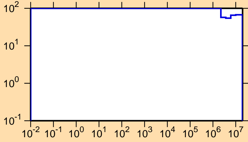
\Delta\sigma/\sigma vs. E for ^{170}\text{Re}(n,p)
