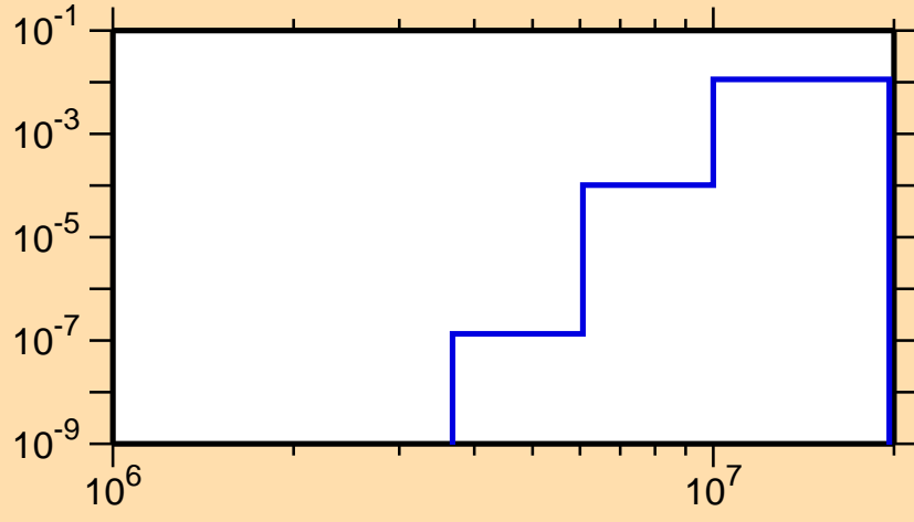
\sigma vs. E for ^{170}\text{Re}(n,d)
