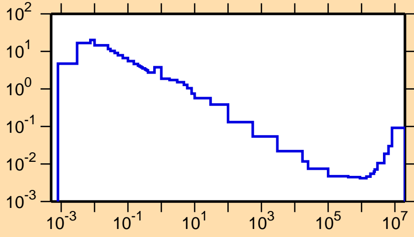
\sigma vs. E for ^{170}\text{Re}(n,\alpha)
