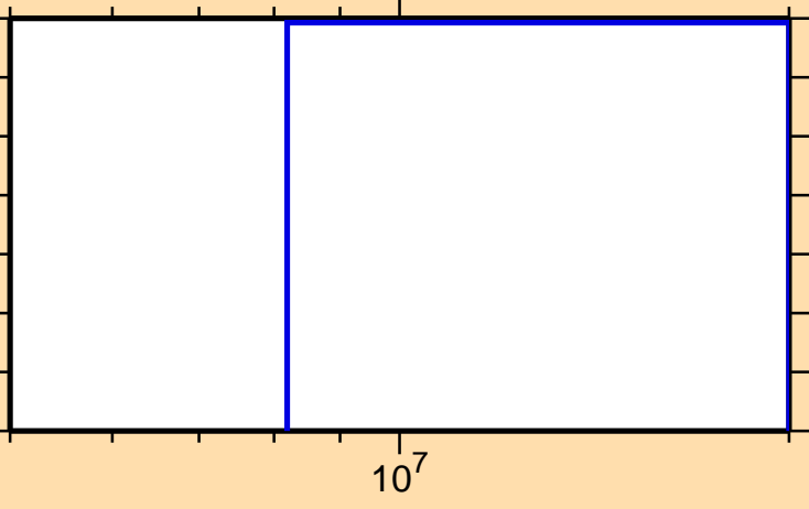
\sigma vs. E for ^{170}\text{Re}(n,3n)
