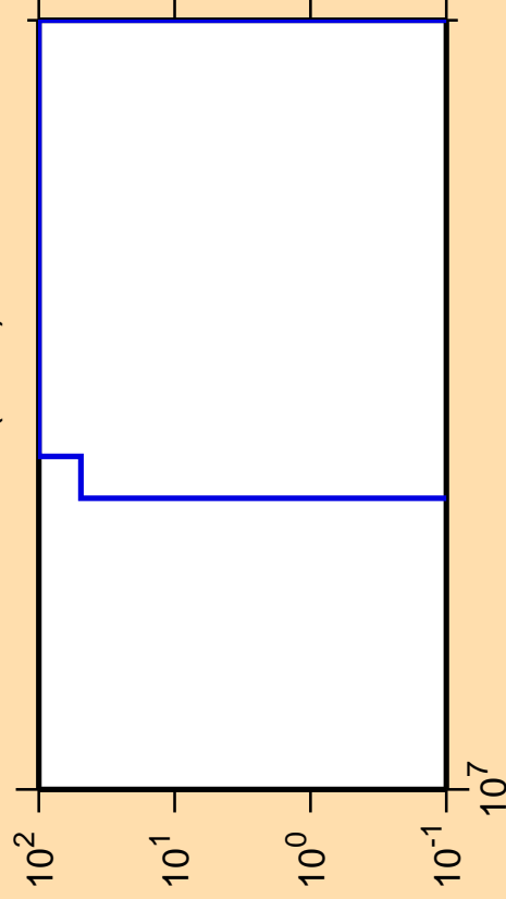
\Delta\sigma/\sigma vs. E for ^{171}\text{Re}(n,nd)
