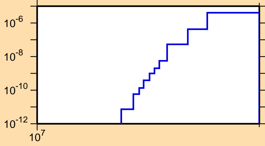
\sigma vs. E for ^{171}\text{Re}(n,nd)
