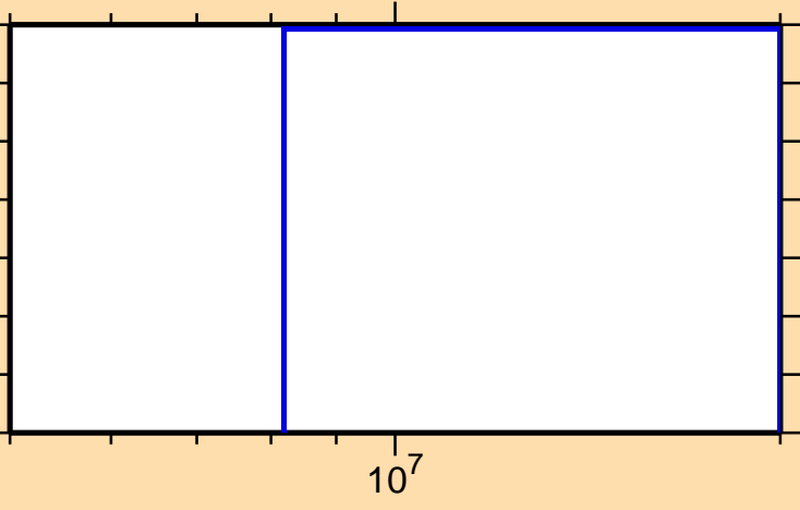
\sigma vs. E for ^{171}\text{Re}(\text{mt117})
