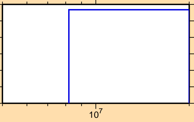
\sigma vs. E for ^{171}\text{Re}(n,\text{nd})
