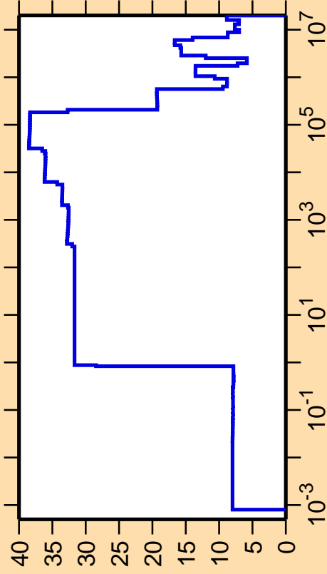
\Delta\sigma/\sigma vs. E for ^{172}\text{Re}(n,\text{el.})
