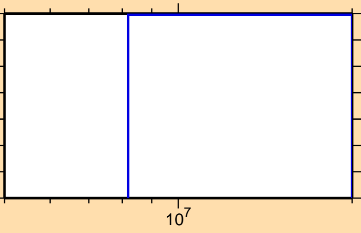
\sigma vs. E for ^{172}\text{Re}(n,2np)
