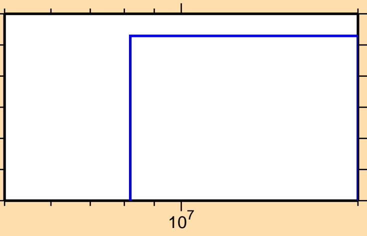
\sigma vs. E for ^{172}\text{Re}(n,3n)
