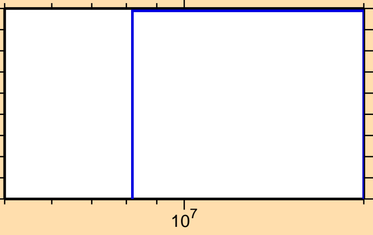
\sigma vs. E for ^{172}\text{Re}(n,\text{nd})
