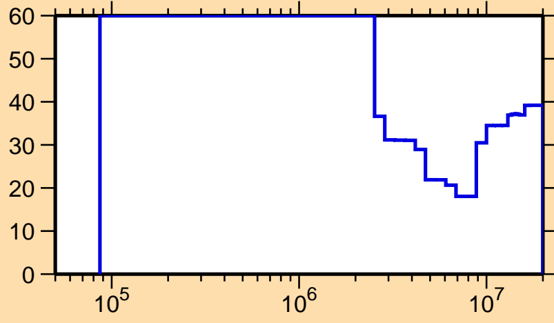
\Delta\sigma/\sigma vs. E for ^{172}\text{Re}(n,n\text{cont.})
