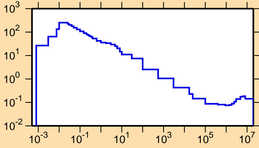
\sigma vs. E for ^{172}\text{Re}(n,p)
