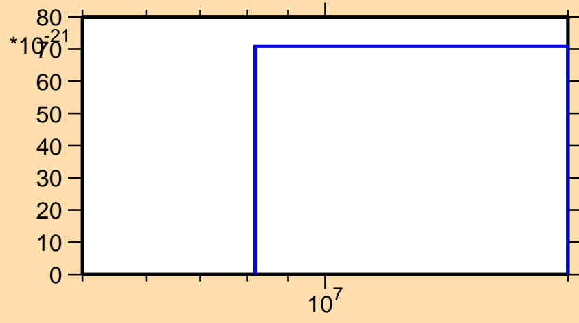
\sigma vs. E for ^{172}\text{Re}(\text{mt } 42)
