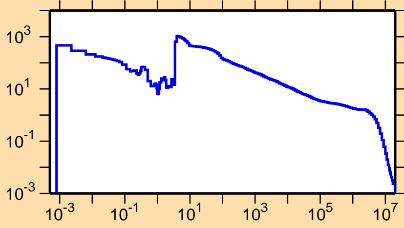
\sigma vs. E for ^{173}\text{Re}(n,\gamma)
