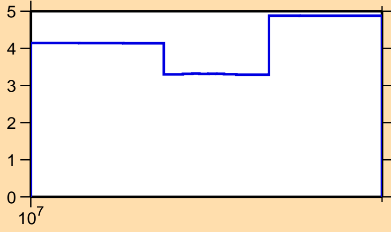
\Delta\sigma/\sigma vs. E for ^{173}\text{Re}(n,\text{el.})
