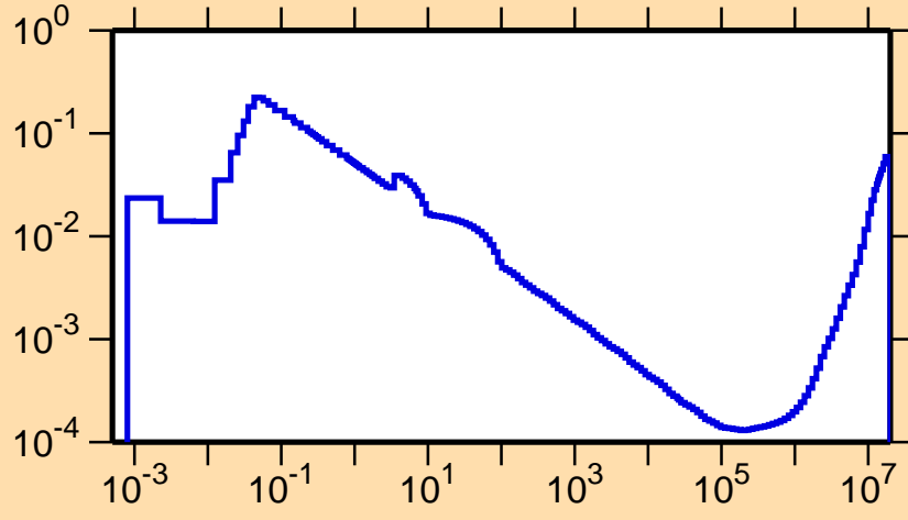
\sigma vs. E for ^{173}\text{Re}(n,\alpha)
