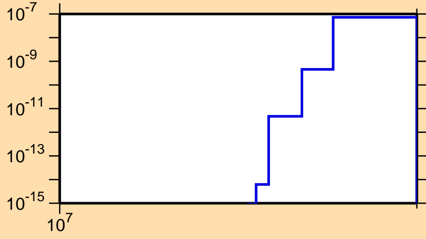
\sigma vs. E for ^{173}\text{Re}(n,nt)
