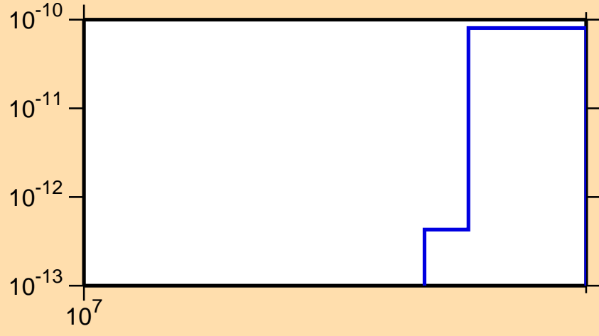
\sigma vs. E for ^{173}\text{Re}(n,\text{pt})
