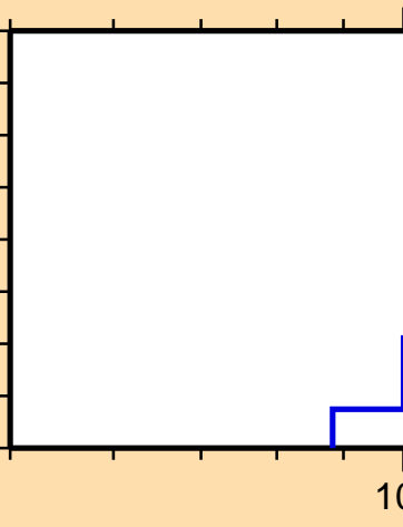
\sigma vs. E for ^{174}\text{Re}(\text{mt117})
