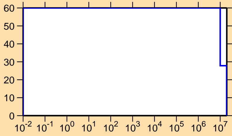
\Delta\sigma/\sigma vs. E for ^{174}\text{Re}(n,p)
