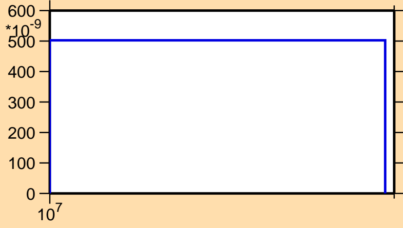
\sigma vs. E for ^{174}\text{Re}(n,3n)
