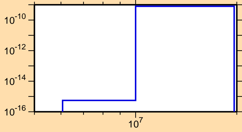
\sigma vs. E for ^{174}\text{Re}(\text{mt117})
