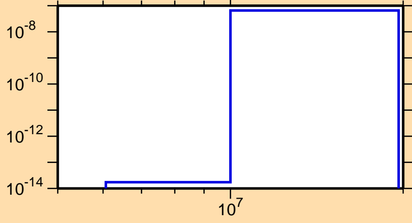
\sigma vs. E for ^{174}\text{Re}(\text{mt } 45)
