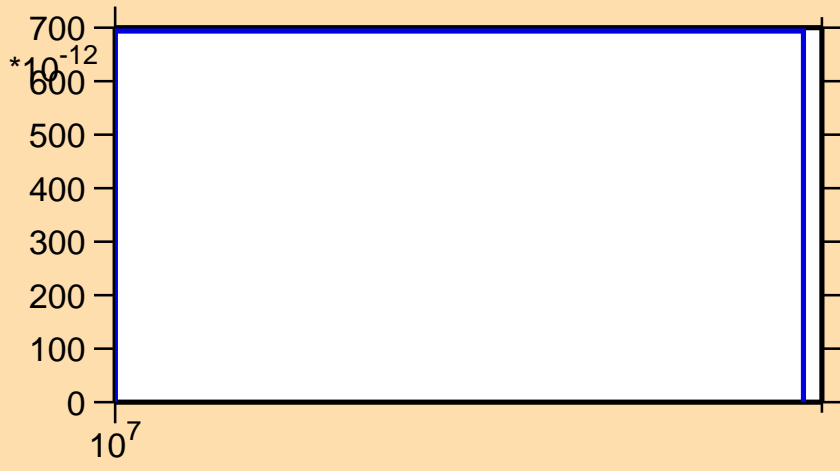
\sigma vs. E for ^{174}\text{Re}(n,\text{pd})
