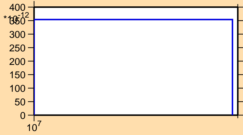
\sigma vs. E for ^{174}\text{Re}(n,nt)
