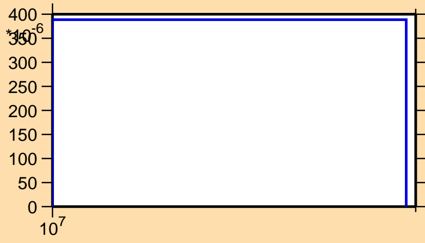
\sigma vs. E for ^{174}\text{Re}(n,2np)
