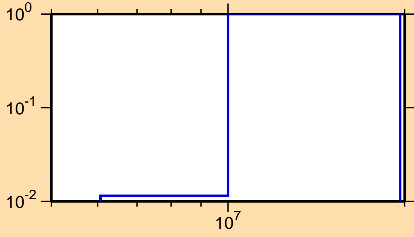
\sigma vs. E for ^{174}\text{Re}(n,2n)
