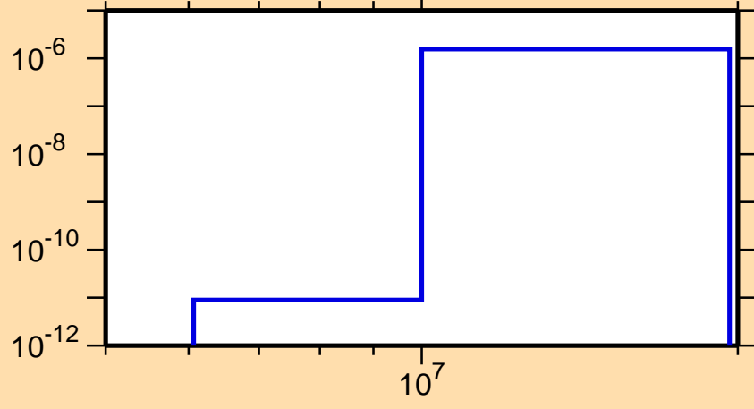
\sigma vs. E for ^{174}\text{Re}(n,\text{He}3)
