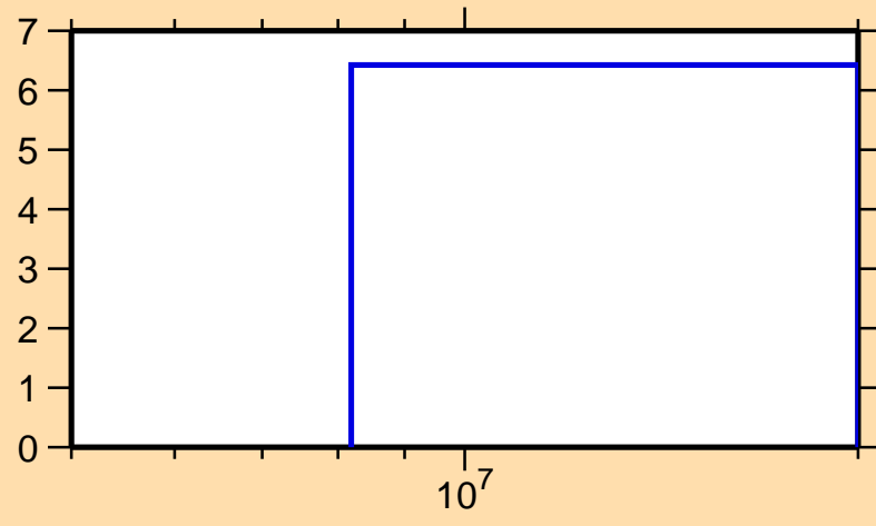
\Delta\sigma/\sigma vs. E for ^{174}\text{Re}(n,\text{el.})
