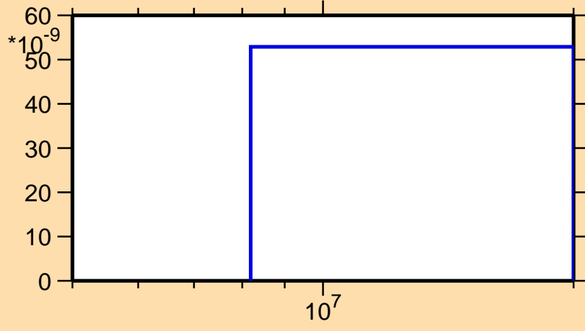
\sigma vs. E for ^{174}\text{Re}(\text{mt } 45)
