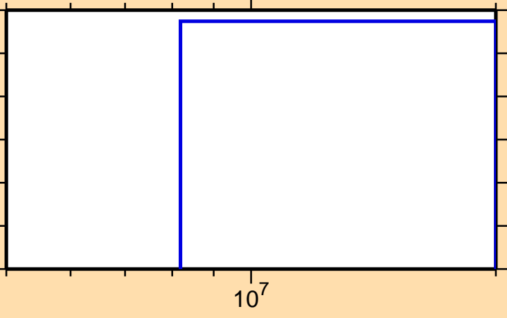
\sigma vs. E for ^{174}\text{Re}(n,\text{pd})
