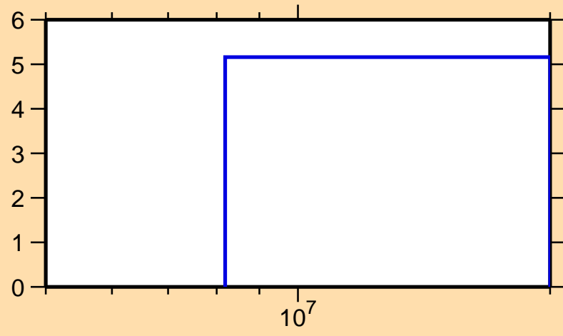
\Delta\sigma/\sigma vs. E for ^{174}\text{Re}(n,\text{tot.})
