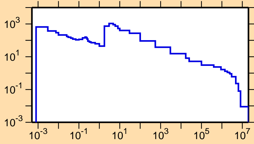
\sigma vs. E for ^{174}\text{Re}(n,\gamma)
