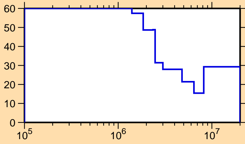
\Delta\sigma/\sigma vs. E for ^{174}\text{Re}(n,n\text{cont.})
