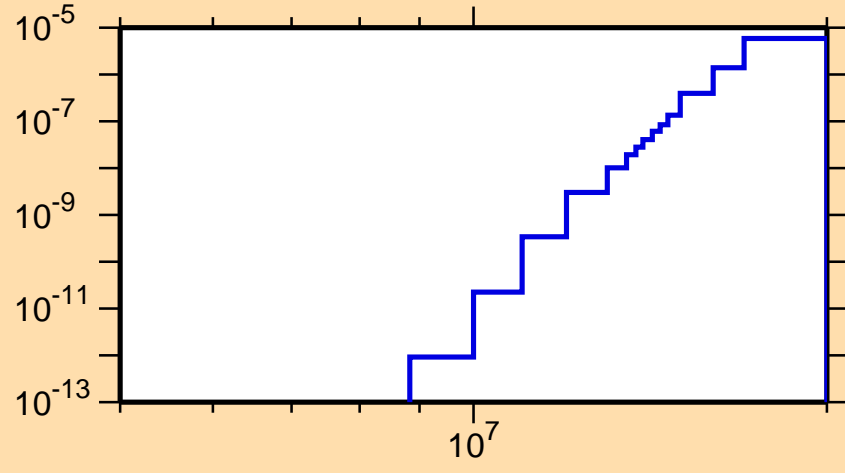
\sigma vs. E for ^{175}\text{Re}(n,\text{He3})
