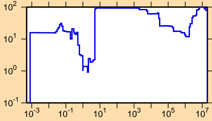
\Delta\sigma/\sigma vs. E for ^{175}\text{Re}(n,\gamma)
