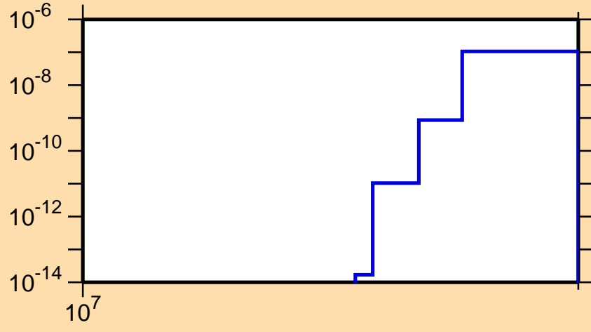
\sigma vs. E for ^{175}\text{Re}(n,nt)
