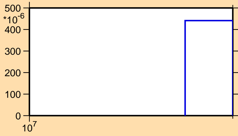
\sigma vs. E for ^{175}\text{Re}(n,3n)
