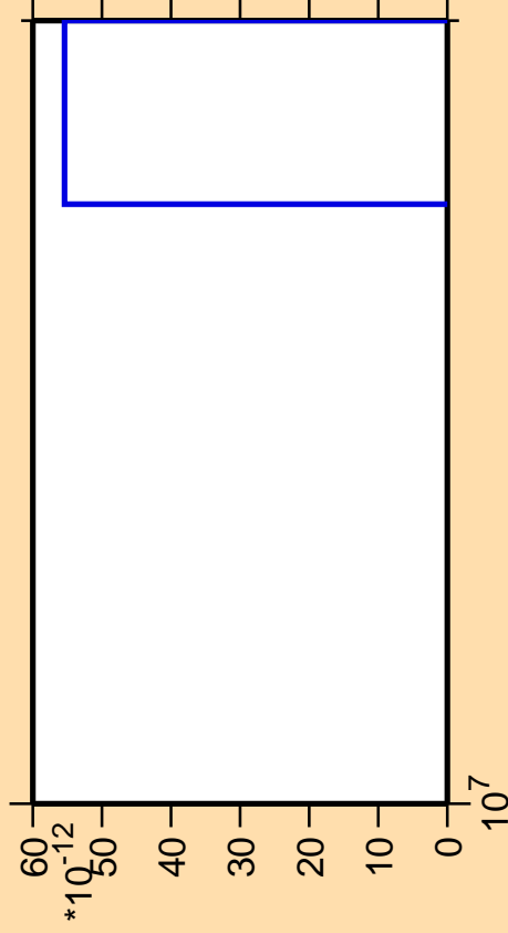
\Delta\sigma/\sigma vs. E for ^{175}\text{Re}(\text{mt } 42)
