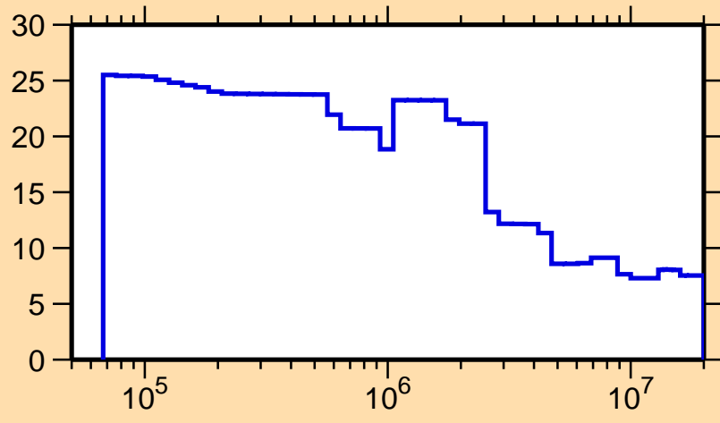
\Delta\sigma/\sigma vs. E for ^{175}\text{Re}(n,\text{nonel.})
