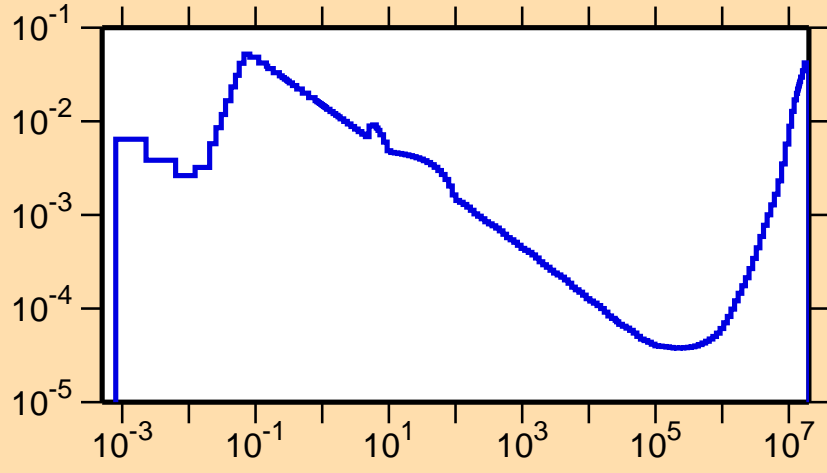
\sigma vs. E for ^{175}\text{Re}(n,\alpha)
