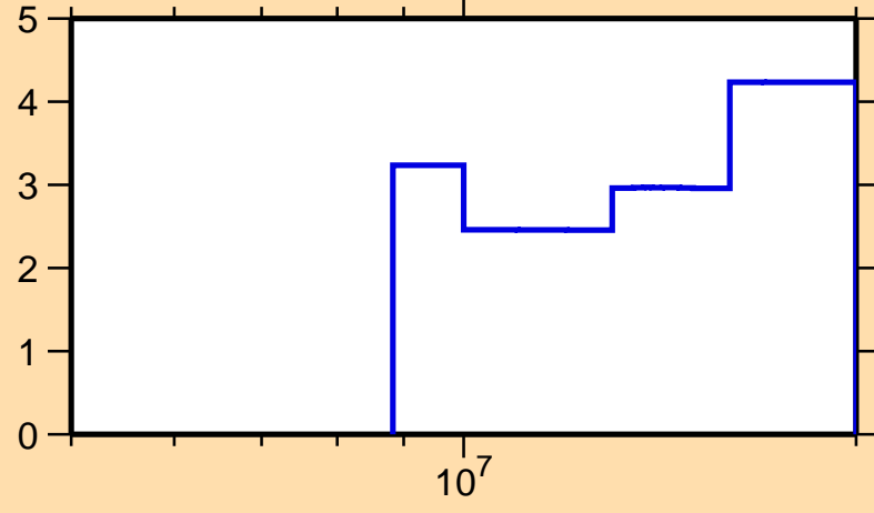
\Delta\sigma/\sigma vs. E for ^{175}\text{Re}(n,\text{tot.})
