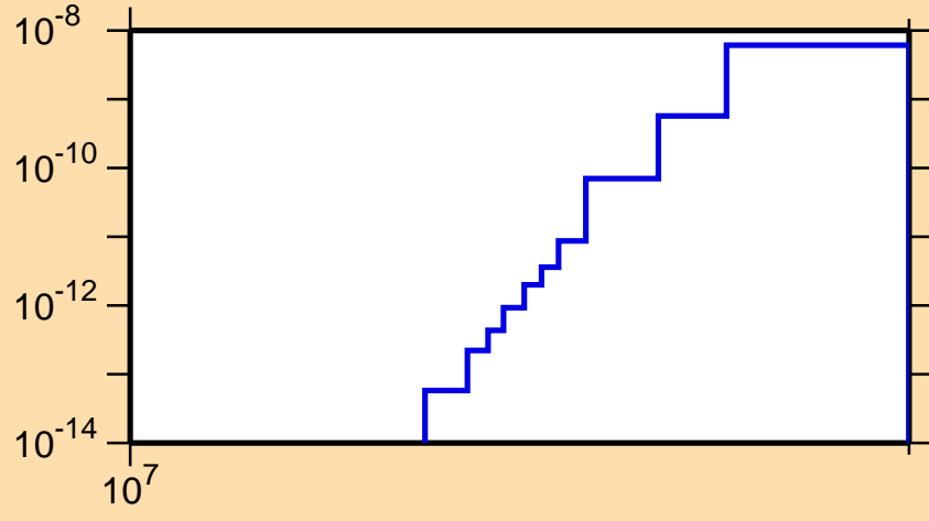
\sigma vs. E for ^{175}\text{Re}(n,\text{pd})
