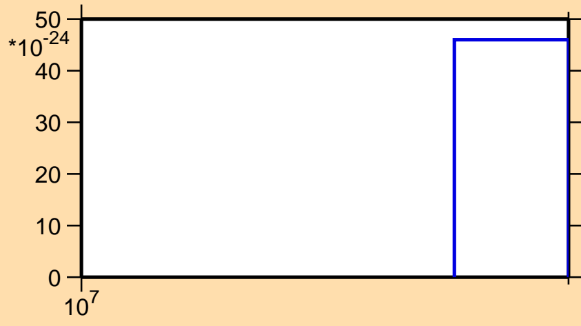
\sigma vs. E for ^{175}\text{Re}(\text{mt } 42)
