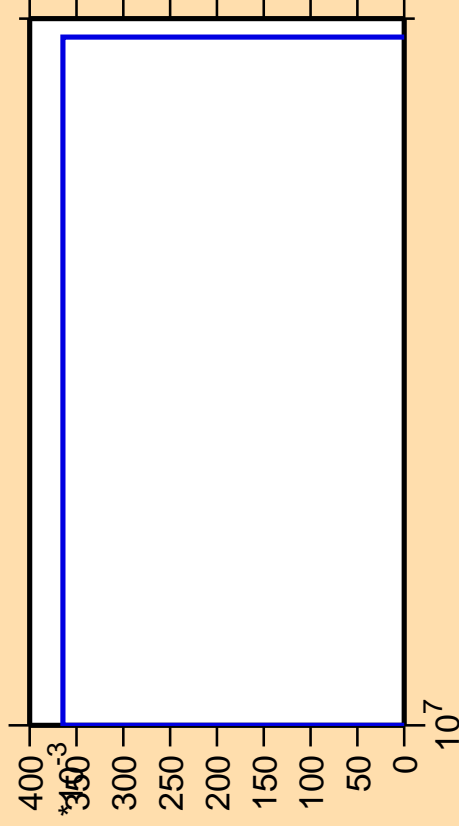
\Delta\sigma/\sigma vs. E for ^{175}\text{Re}(n,\text{pt})
