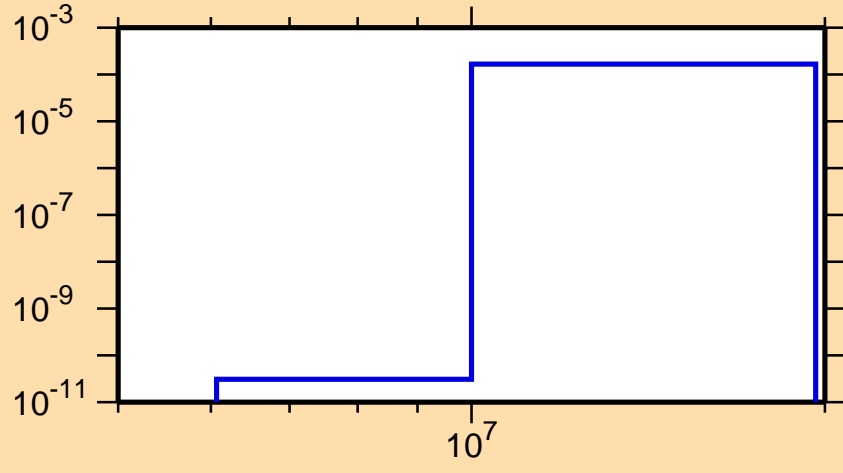
\sigma vs. E for ^{175}\text{Re}(n,t)
