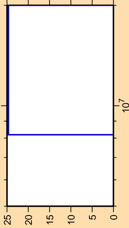
\Delta\sigma/\sigma vs. E for ^{175}\text{Re}(n,2n)
