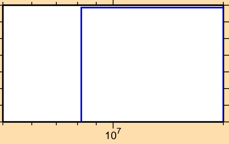
\sigma vs. E for ^{175}\text{Re}(n,\text{nd})
