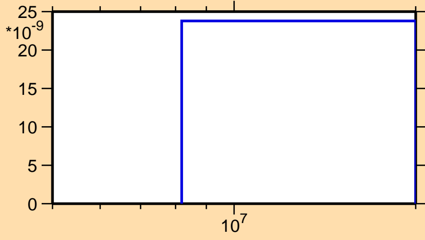
\sigma vs. E for ^{175}\text{Re}(\text{mt } 45)
