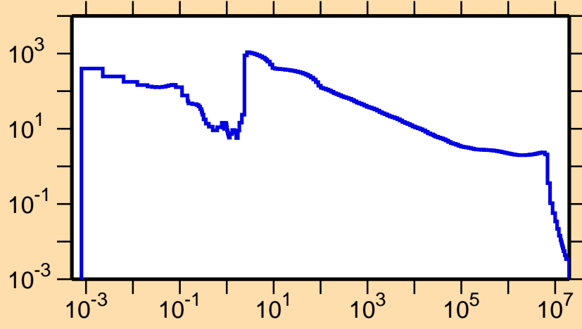
\sigma vs. E for ^{176}\text{Re}(n,\gamma)
