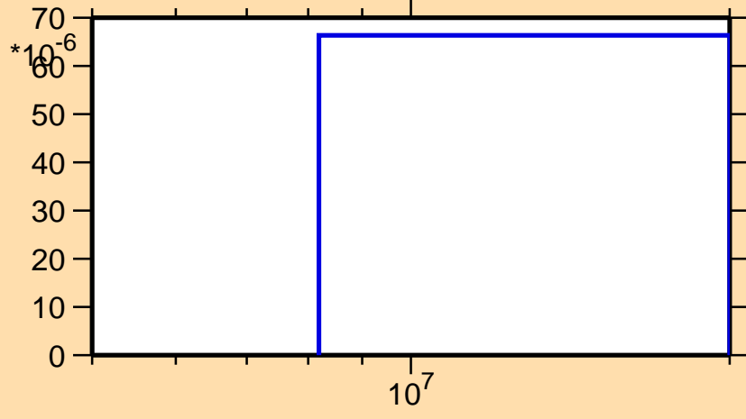
\sigma vs. E for ^{176}\text{Re}(n,2np)
