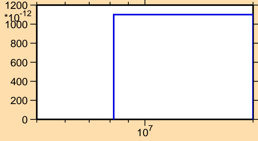
\sigma vs. E for ^{176}\text{Re}(n,nt)
