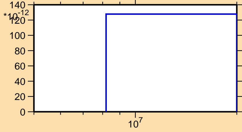
\sigma vs. E for ^{176}\text{Re}(\text{mt117})
