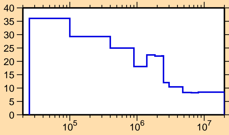
\Delta\sigma/\sigma vs. E for ^{176}\text{Re}(n,\text{nonel.})
