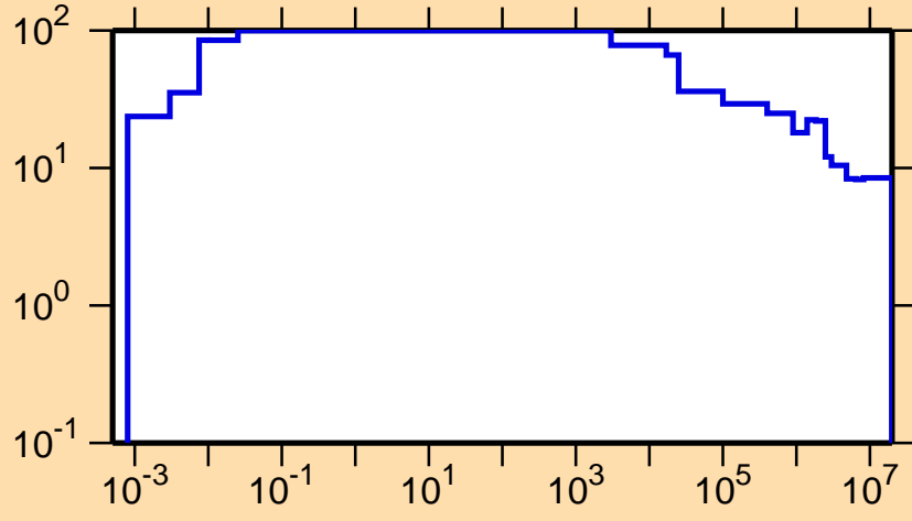
\Delta\sigma/\sigma vs. E for ^{176}\text{Re}(n,\text{nonel.})
