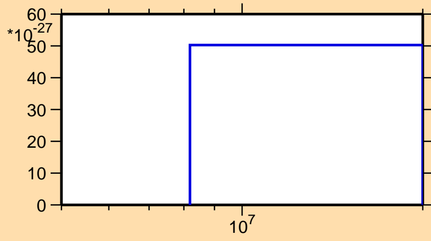
\sigma vs. E for ^{176}\text{Re}(\text{mt } 42)
