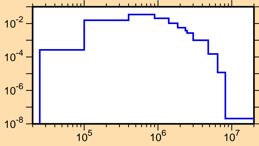
\sigma vs. E for ^{176}\text{Re}(n,n_1)
