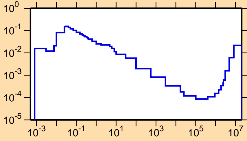
\sigma vs. E for ^{176}\text{Re}(n,\alpha)
