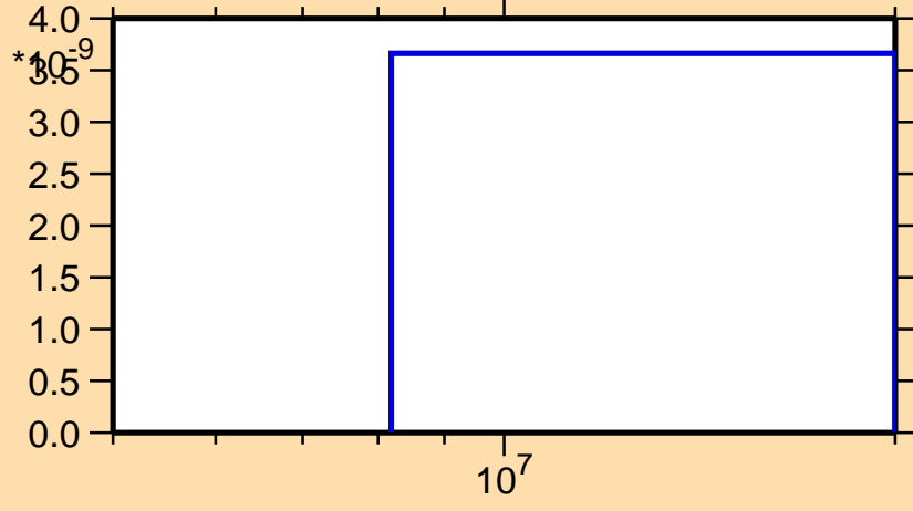
\sigma vs. E for ^{176}\text{Re}(\text{mt } 45)
