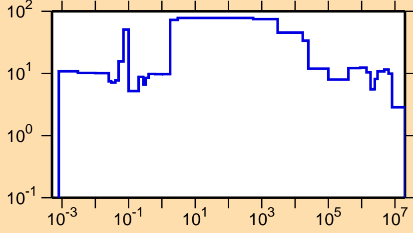
\Delta\sigma/\sigma vs. E for ^{176}\text{Re}(n,\text{tot.})
