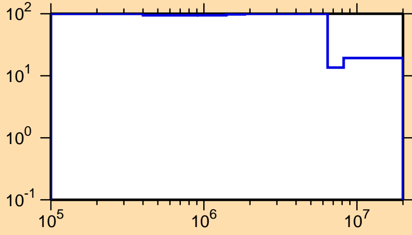
\Delta\sigma/\sigma vs. E for ^{176}\text{Re}(n,n\text{cont.})
