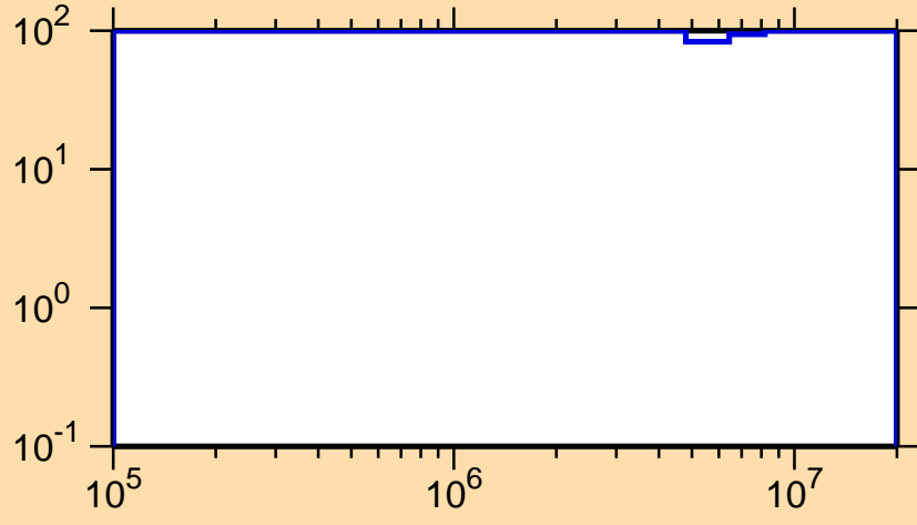
\Delta\sigma/\sigma vs. E for ^{176}\text{Re}(n,n_1)
