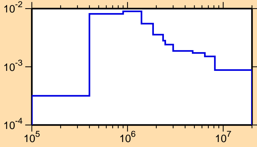
\sigma vs. E for ^{176}\text{Re}(n,n_4)
