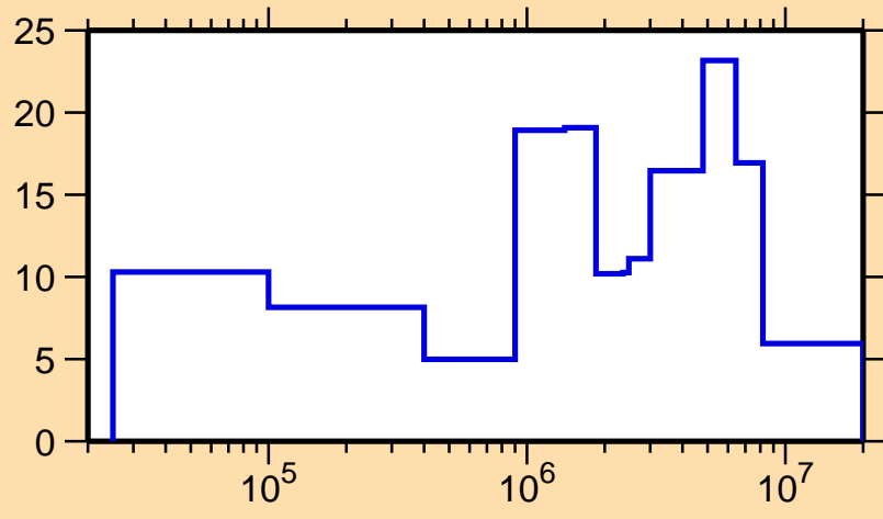
\Delta\sigma/\sigma vs. E for ^{176}\text{Re}(n,\text{el.})
