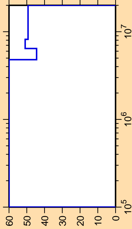
\Delta\sigma/\sigma vs. E for ^{176}\text{Re}(n,n_2)
