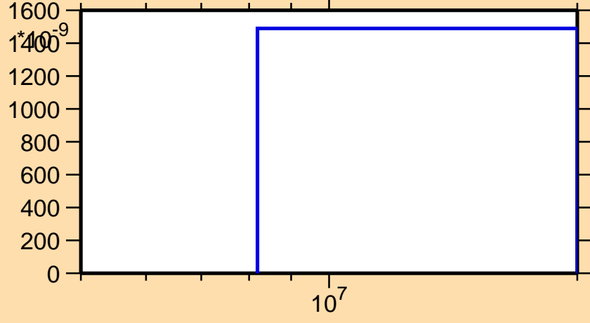
\sigma vs. E for ^{176}\text{Re}(n,2n\alpha)
