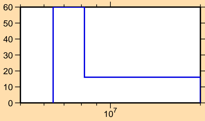
\Delta\sigma/\sigma vs. E for ^{176}\text{Re}(n,2n)
