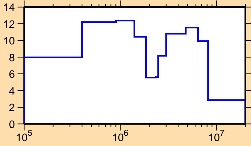
\Delta\sigma/\sigma vs. E for ^{176}\text{Re}(n,\text{tot.})
