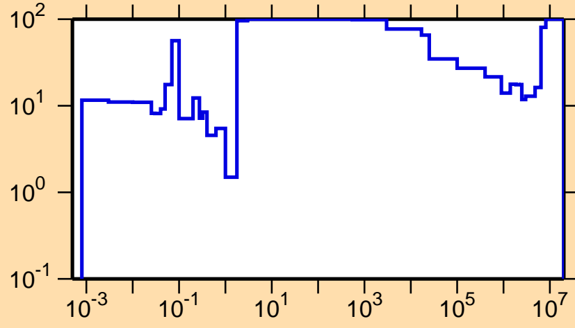
\Delta\sigma/\sigma vs. E for ^{176}\text{Re}(n,\gamma)
