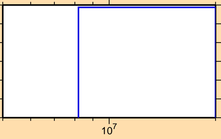
\sigma vs. E for ^{176}\text{Re}(n,\text{nd})
