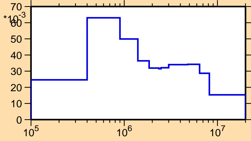
\sigma vs. E for ^{176}\text{Re}(n,n_2)
