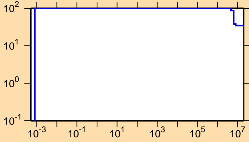
\Delta\sigma/\sigma vs. E for ^{176}\text{Re}(n,p)
