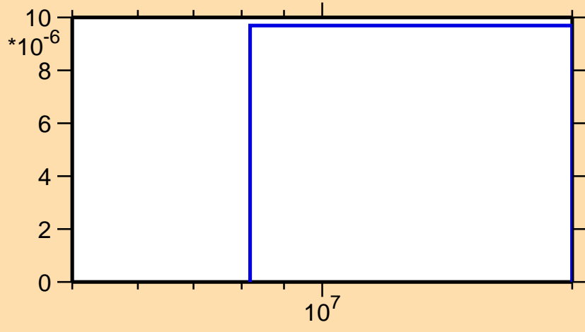
\sigma vs. E for ^{176}\text{Re}(n,3n)
