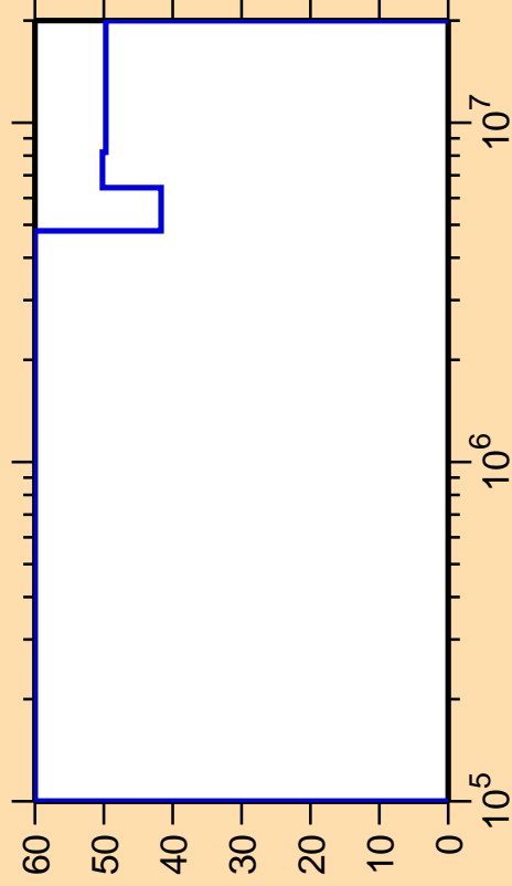
\Delta\sigma/\sigma vs. E for ^{176}\text{Re}(n,n_4)
