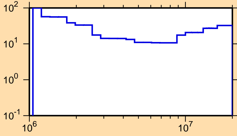
\Delta\sigma/\sigma vs. E for ^{177}\text{Re}(n,n\text{cont.})
