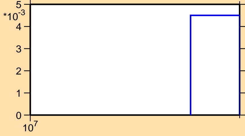
\sigma vs. E for ^{177}\text{Re}(n,3n)
