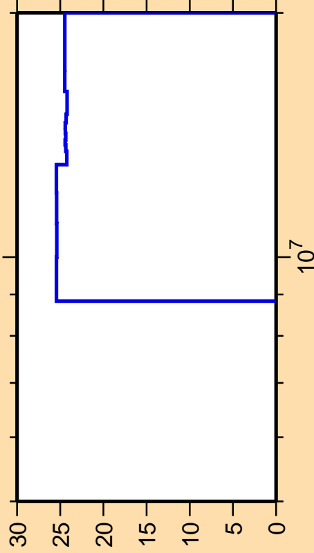
\Delta\sigma/\sigma vs. E for ^{177}\text{Re}(n,n_1)
