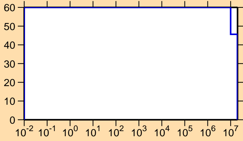
\Delta\sigma/\sigma vs. E for ^{177}\text{Re}(n,p)
