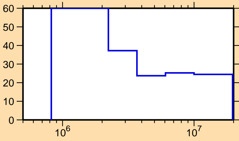
\Delta\sigma/\sigma vs. E for ^{177}\text{Re}(n,n_1)
