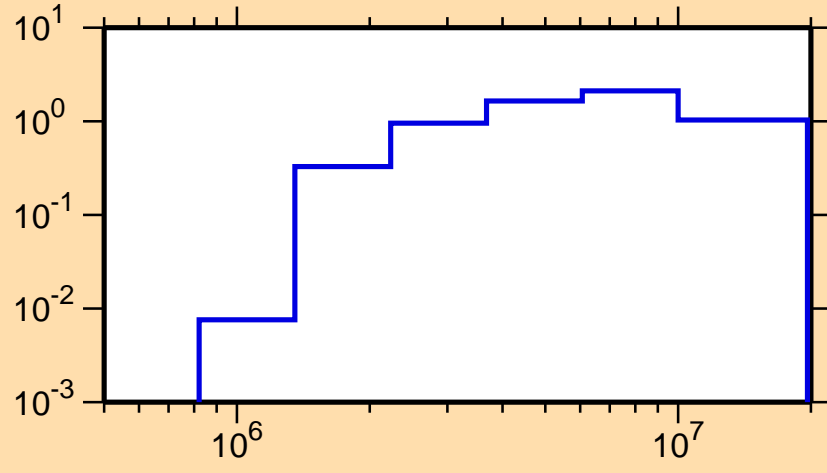
\sigma vs. E for ^{177}\text{Re}(n,n\text{cont.})
