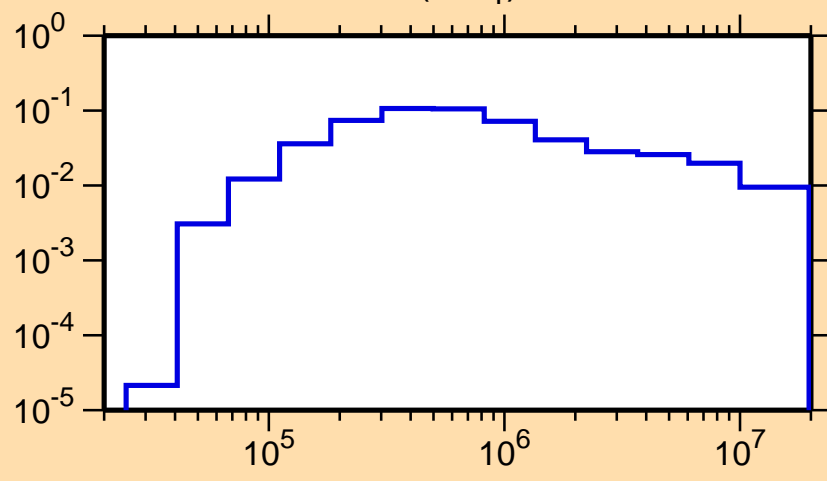
\sigma vs. E for ^{177}\text{Re}(n,n_1)
