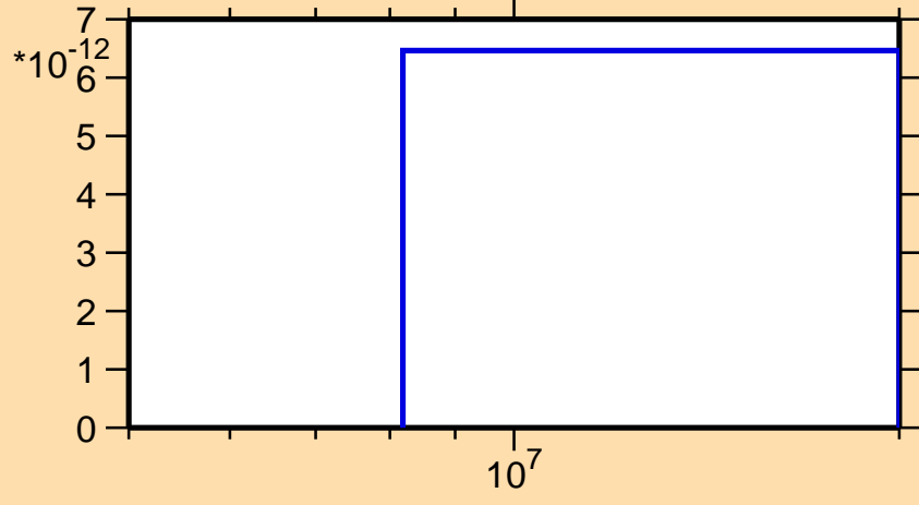
\sigma vs. E for ^{177}\text{Re}(n,pd)
