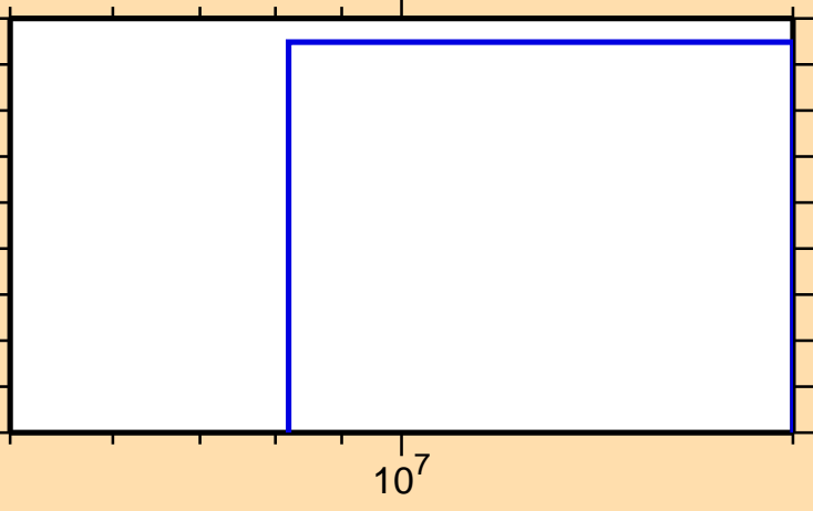
\sigma vs. E for ^{177}\text{Re}(n,2np)
