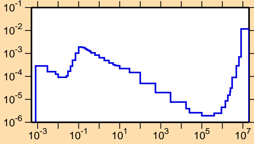
\sigma vs. E for ^{177}\text{Re}(n,\alpha)
