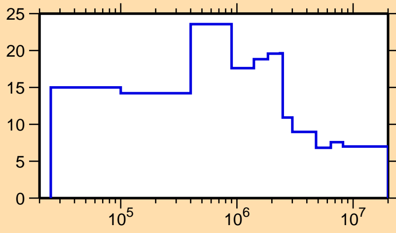
\Delta\sigma/\sigma vs. E for ^{177}\text{Re}(n,\text{nonel.})
