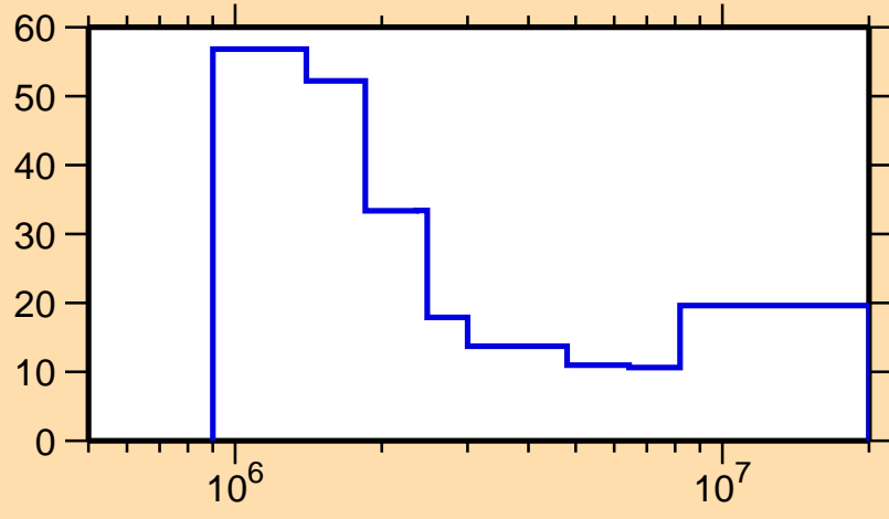
\Delta\sigma/\sigma vs. E for ^{177}\text{Re}(n,n\text{cont.})
