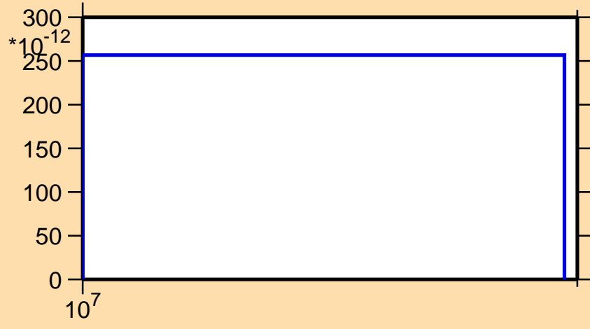
\sigma vs. E for ^{178}\text{Re}(\text{mt } 45)
