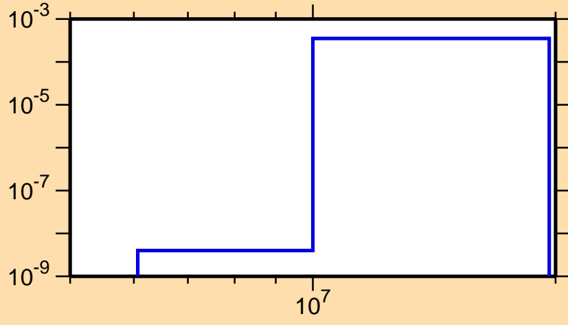
\sigma vs. E for ^{178}\text{Re}(n,t)
