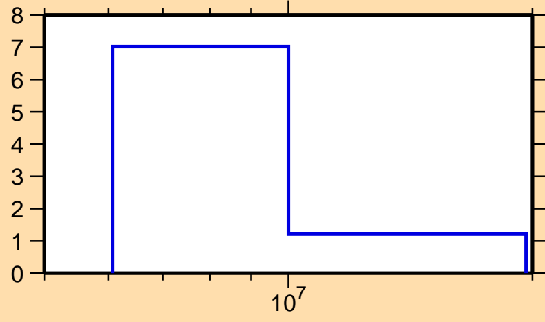
\Delta\sigma/\sigma vs. E for ^{178}\text{Re}(n,\text{tot.})
