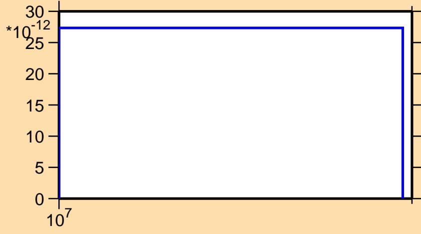
\sigma vs. E for ^{178}\text{Re}(\text{mt117})
