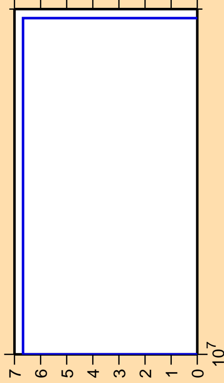
\Delta\sigma/\sigma vs. E for ^{178}\text{Re}(n,pd)
