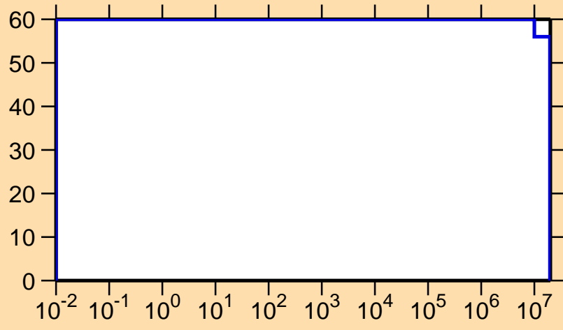
\Delta\sigma/\sigma vs. E for ^{178}\text{Re}(n,p)
