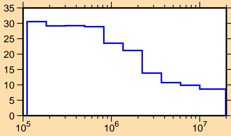
\Delta\sigma/\sigma vs. E for ^{178}\text{Re}(n,n\text{onel.})
