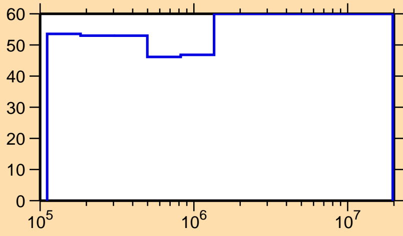
\Delta\sigma/\sigma vs. E for ^{178}\text{Re}(n,n_1)
