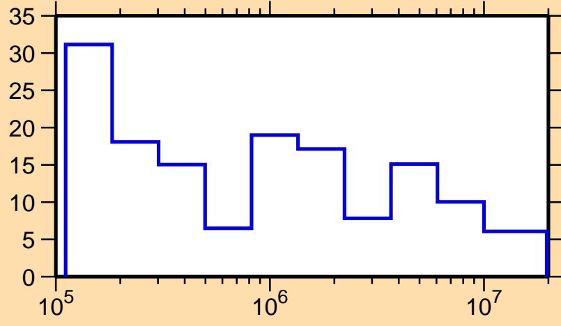
\Delta\sigma/\sigma vs. E for ^{178}\text{Re}(n, el.)
