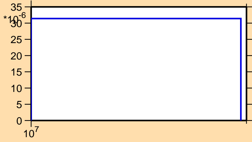
\sigma vs. E for ^{178}\text{Re}(n,2np)
