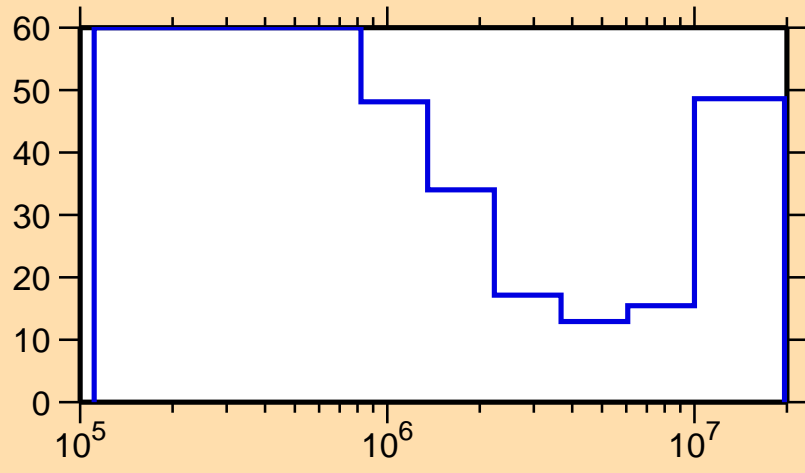
\Delta\sigma/\sigma vs. E for ^{178}\text{Re}(n,n\text{cont.})
