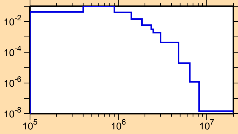
\sigma vs. E for ^{178}\text{Re}(n,n_1)
