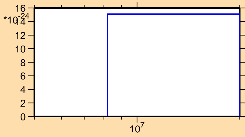
\sigma vs. E for ^{178}\text{Re}(\text{mt } 42)
