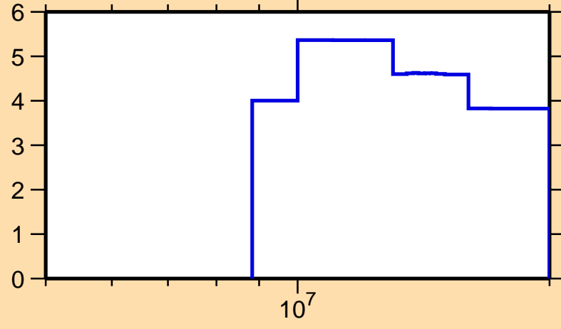
\Delta\sigma/\sigma vs. E for ^{179}\text{Re}(n,\text{el.})
