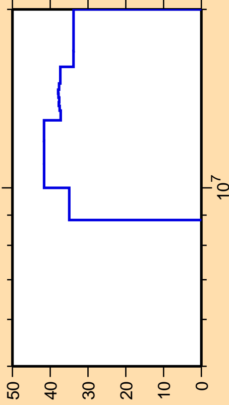
\Delta\sigma/\sigma vs. E for ^{179}\text{Re}(n,n\text{cont.})
