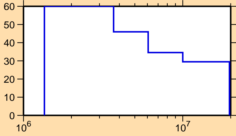
\Delta\sigma/\sigma vs. E for ^{179}\text{Re}(n,n_1)
