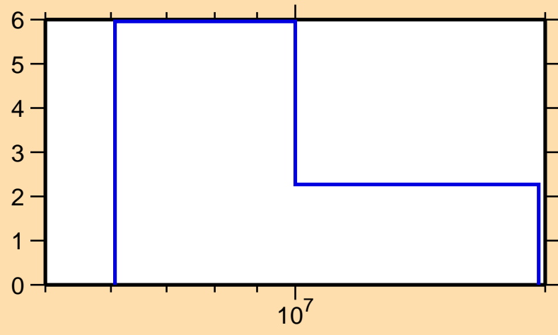
\Delta\sigma/\sigma vs. E for ^{179}\text{Re}(n,\text{tot.})
