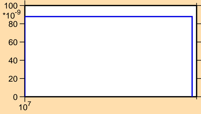
\sigma vs. E for ^{179}\text{Re}(n,nd)
