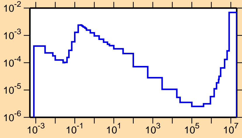
\sigma vs. E for ^{179}\text{Re}(n,\alpha)
