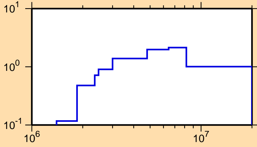
\sigma vs. E for ^{179}\text{Re}(n,n\text{cont.})
