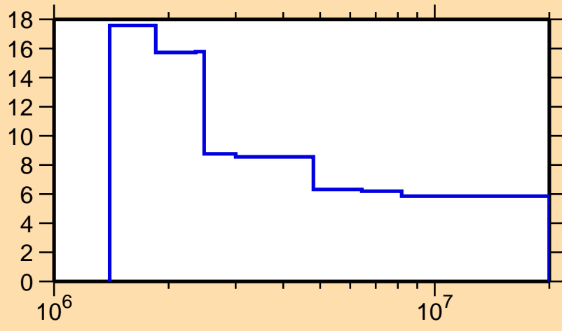
\Delta\sigma/\sigma vs. E for ^{179}\text{Re}(n,n\text{onel.})
