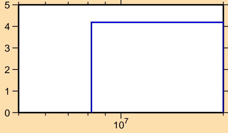
\Delta\sigma/\sigma vs. E for ^{179}\text{Re}(n,2n)
