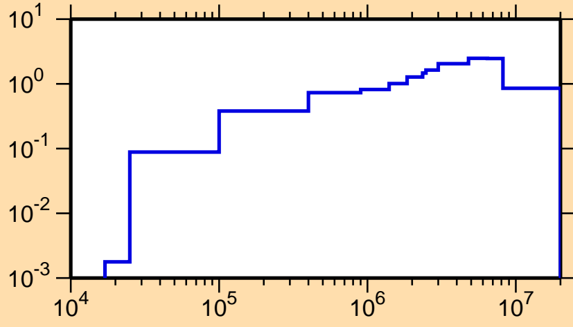
\sigma vs. E for ^{180}\text{Re}(n,\text{inel.})
