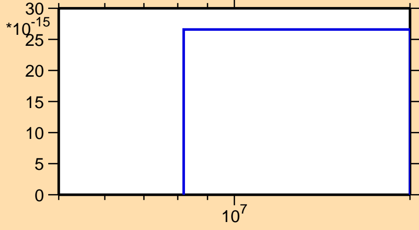
\sigma vs. E for ^{180}\text{Re}(n,pd)
