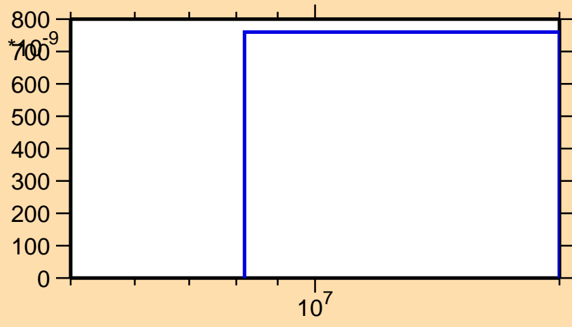
\sigma vs. E for ^{180}\text{Re}(n,2n\alpha)
