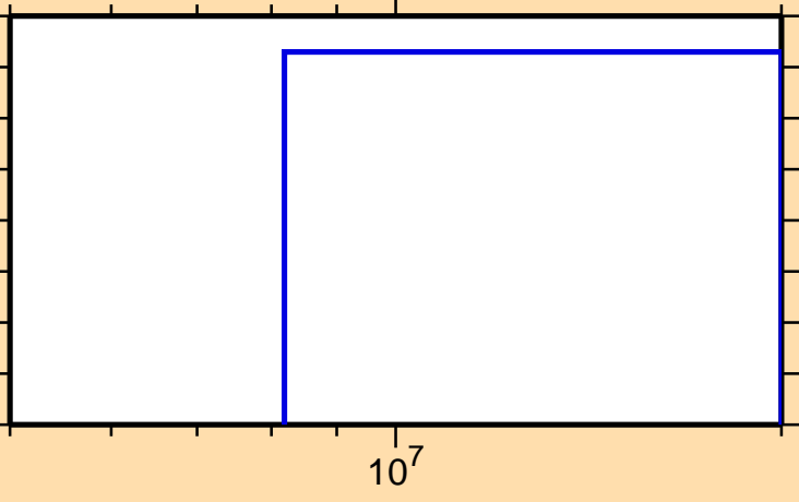
\sigma vs. E for ^{180}\text{Re}(n,\text{nd})
