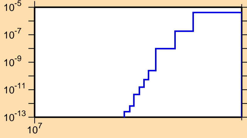
\sigma vs. E for ^{181}\text{Re}(n,nd)
