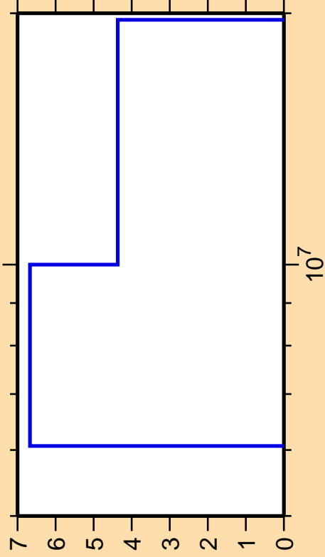
\Delta\sigma/\sigma vs. E for ^{181}\text{Re}(n,2n)
