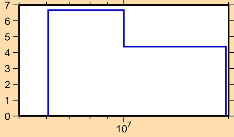
\Delta\sigma/\sigma vs. E for ^{181}\text{Re}(n,2n)
