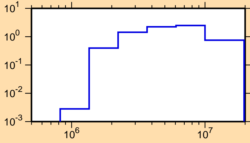
\sigma vs. E for ^{181}\text{Re}(n,n\text{cont.})
