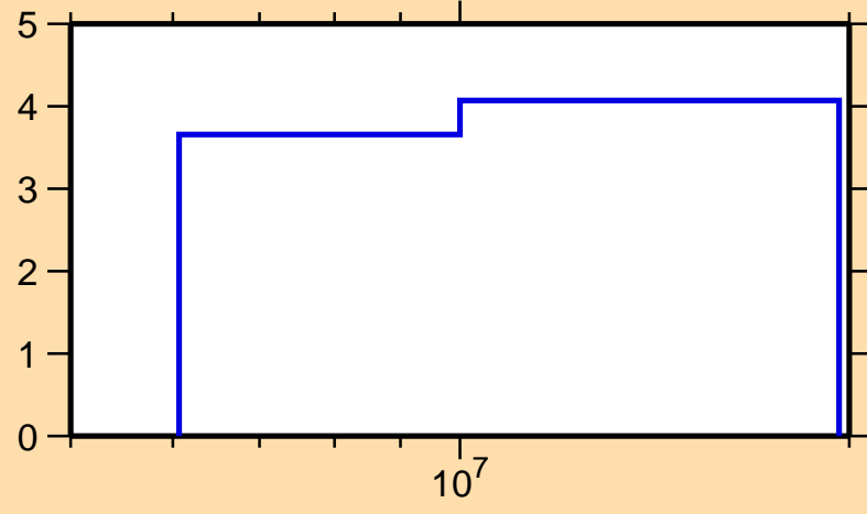
\Delta\sigma/\sigma vs. E for ^{181}\text{Re}(n,\text{nonel.})
