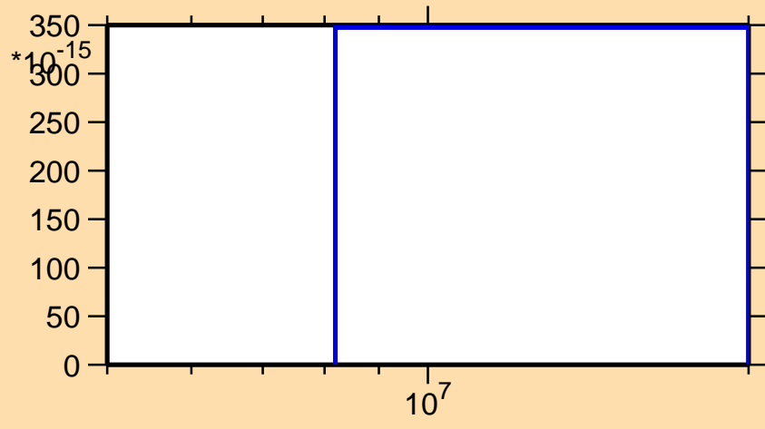
\sigma vs. E for ^{181}\text{Re}(\text{mt117})
