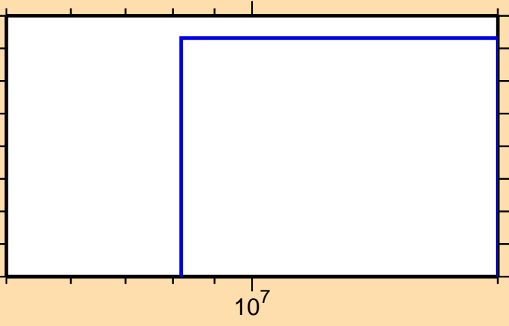
\sigma vs. E for ^{181}\text{Re}(n,2np)
