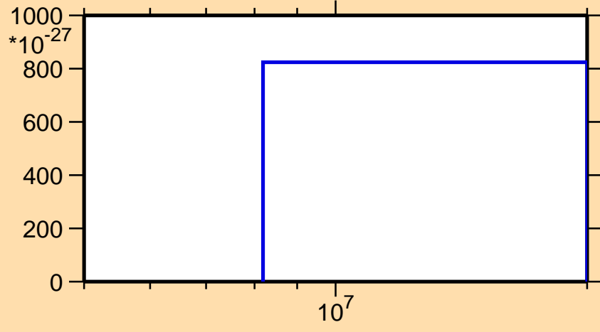
\sigma vs. E for ^{181}\text{Re}(\text{mt } 42)
