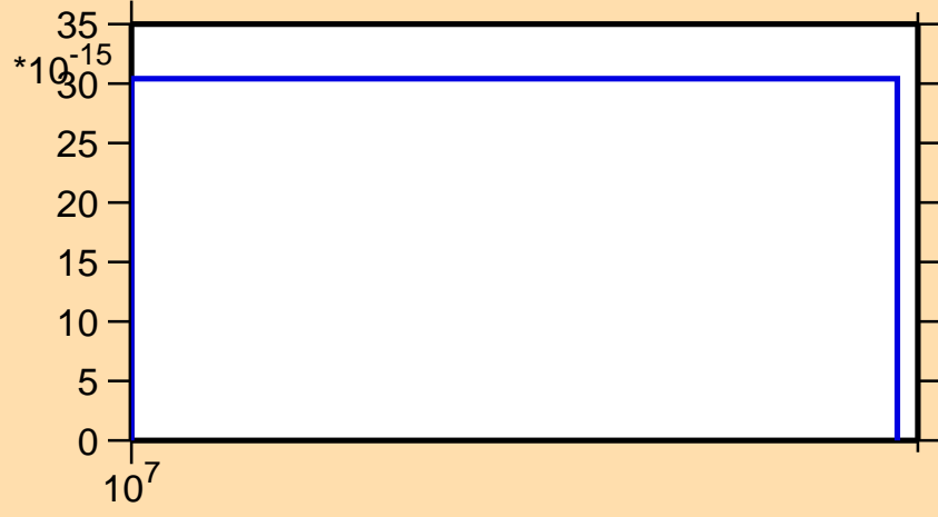
\sigma vs. E for ^{182}\text{Re} (mt 45)
