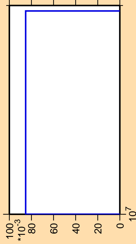
\Delta\sigma/\sigma vs. E for ^{182}\text{Re} (mt 45)
