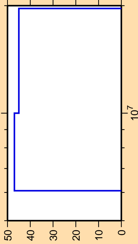
\Delta\sigma/\sigma vs. E for ^{182}\text{Re}(n,\gamma)
