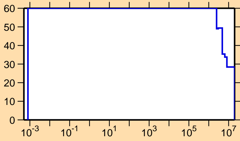
\Delta\sigma/\sigma vs. E for ^{182}\text{Re}(n,p)
