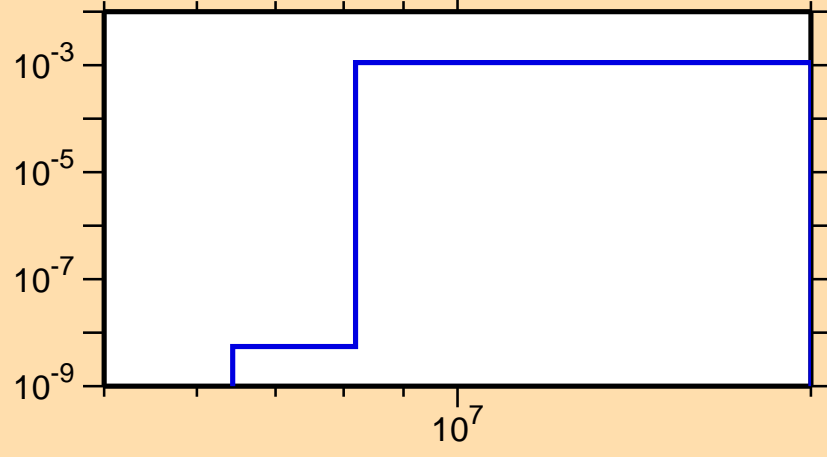
\sigma vs. E for ^{182}\text{Re}(n,np)
