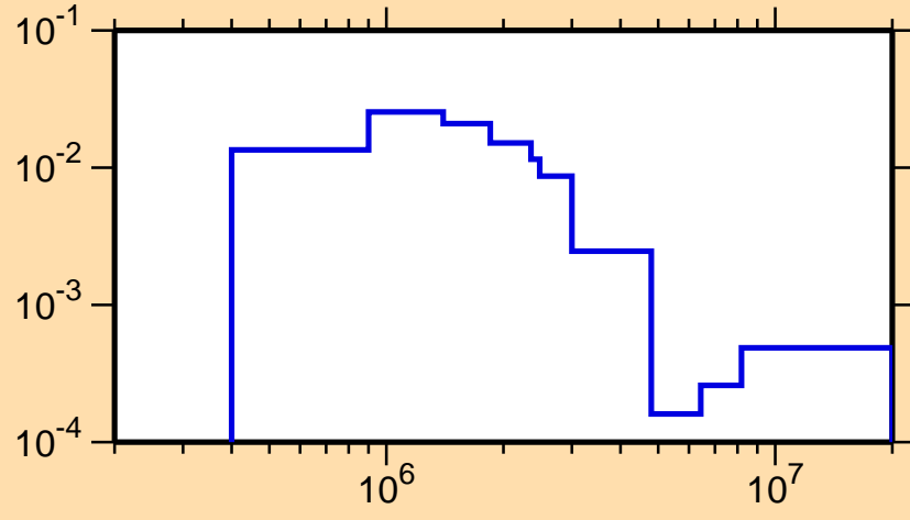
\sigma vs. E for ^{182}\text{Re}(n,n_4)
