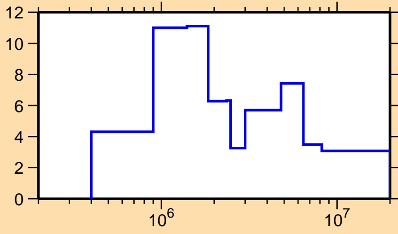
\Delta\sigma/\sigma vs. E for ^{182}\text{Re}(n, el.)
