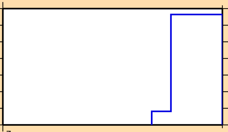
\sigma vs. E for ^{182}\text{Re}(\text{mt } 45)
