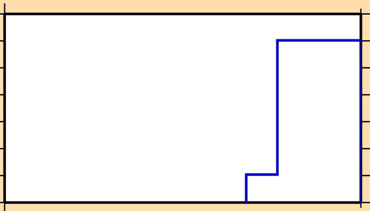
\sigma vs. E for ^{182}\text{Re}(\text{mt117})
