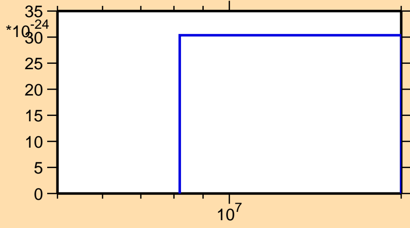
\sigma vs. E for ^{182}\text{Re} (mt 42)
