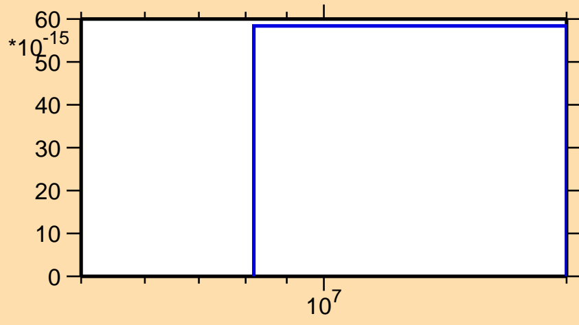
\sigma vs. E for ^{182}\text{Re}(\text{mt117})
