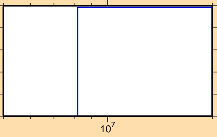
\sigma vs. E for ^{182}\text{Re}(n,2np)
