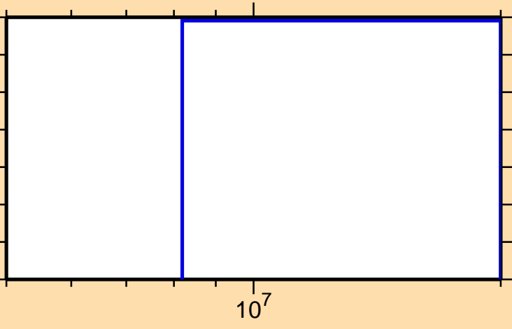
\sigma vs. E for ^{182}\text{Re}(n,\text{He3})
