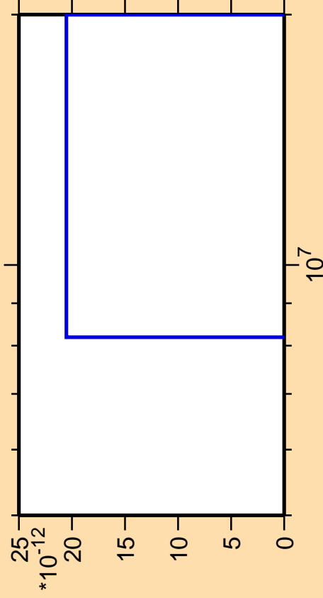
\Delta\sigma/\sigma vs. E for ^{182}\text{Re} (mt 42)
