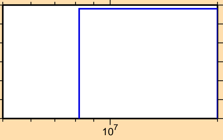
\sigma vs. E for ^{182}\text{Re}(n,nt)
